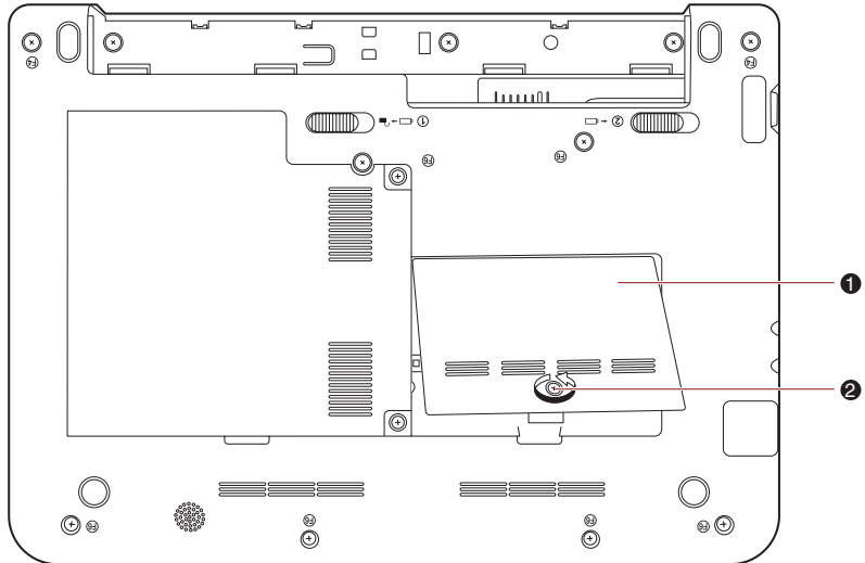
Figure 8-3 Seating the memory module cover
