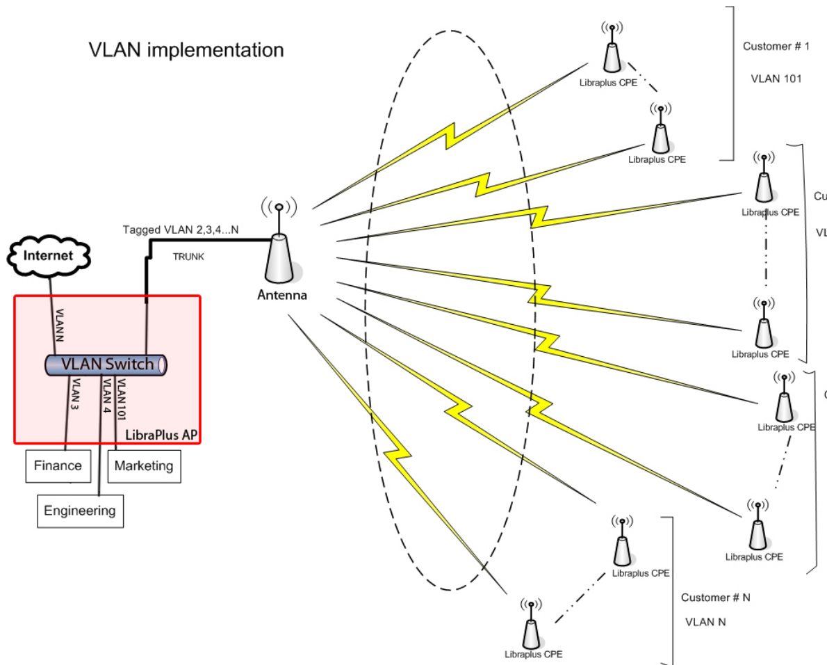
Fig. 4.1. Multipoint VLAN Configuration
