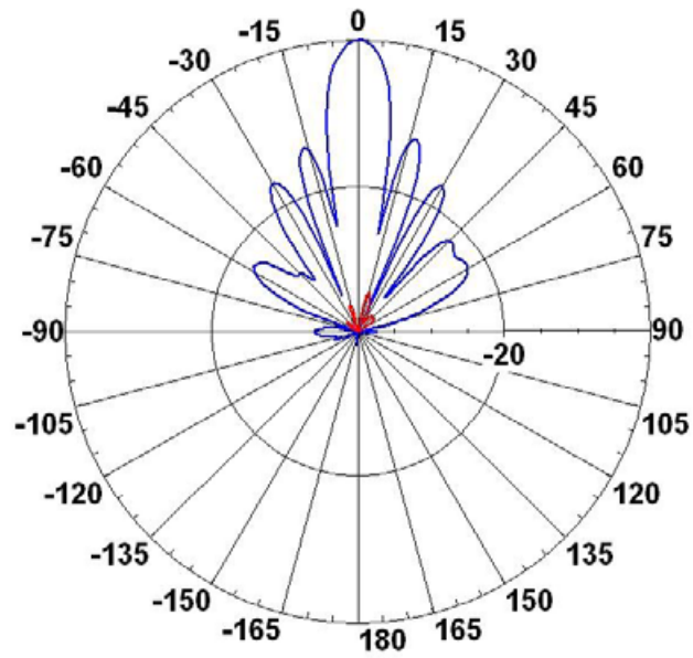
Fig. 8.1. Azimuth Radiation Pattern Midband Freq. 5.45 GHz
