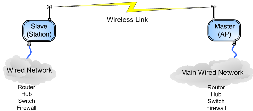
Fig. 2.14. Point-to-Point Wireless Bridge
