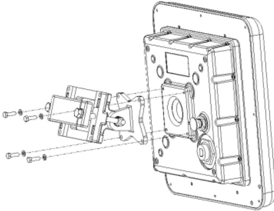
Fig. 3.2. LibraPlus Assembly Diagram
