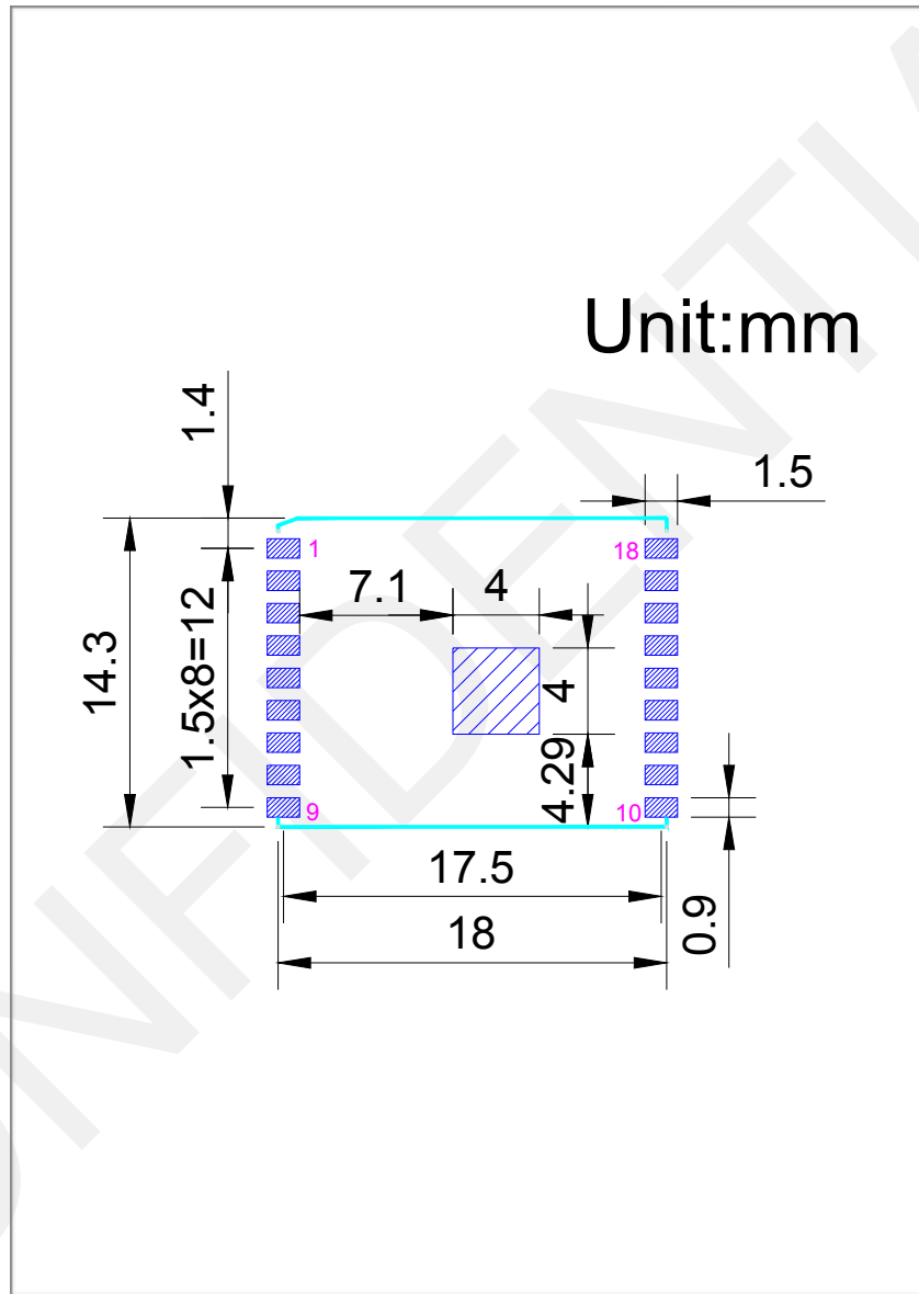
Figure 6-1. Recommended PCB Land Pattern of ESP-WROOM-02UC
