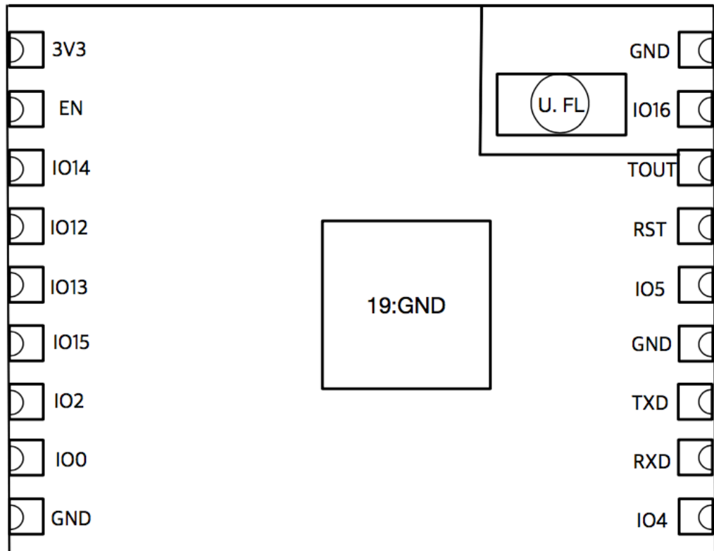
Figure 2-1. ESP-WROOM-02UC Pin Layout (Top View)
