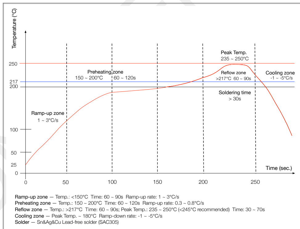
Figure 4-1. ESP-WROOM-02UC Reflow Profile
