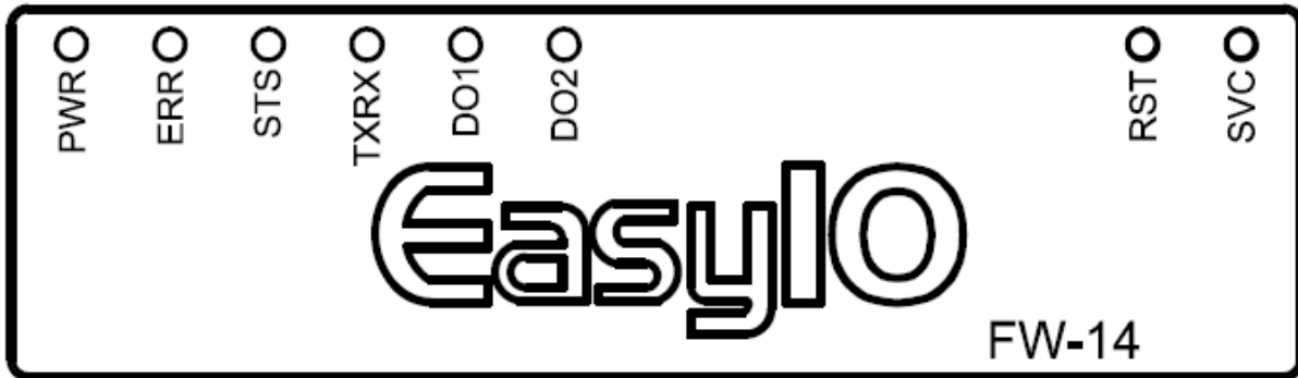
Image shows the Status indicator, Error indicator and individual Digital Output indicator Button and LED indications. Image shown is an EasyIO FW-14.
