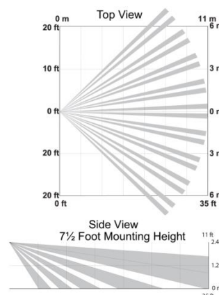
Figure 7: High Sensitivity Setting
