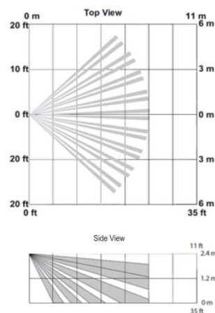
Figure 7: High Sensitivity Setting
