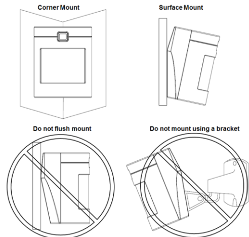
Figure 3: Wall Mount Options
