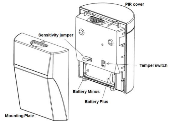
Figure 8: PIR Components, Battery Locations & Tamper Switch
