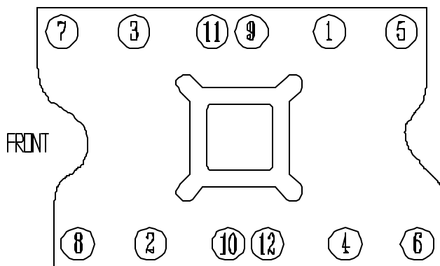
Ford 351C Intake Manifold Tightening Sequence
