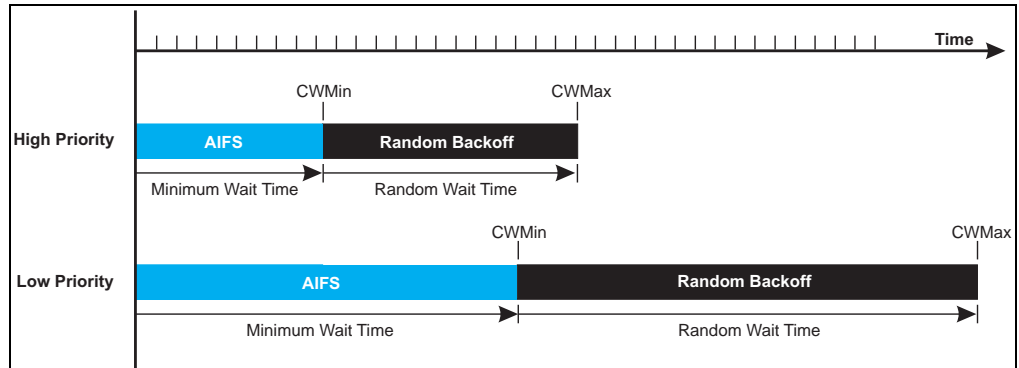
Figure 45: WMM Backoff Wait Times
