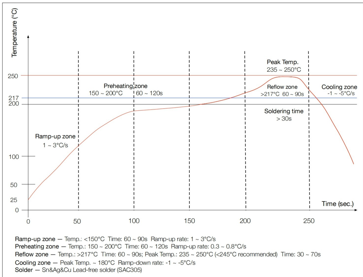
Figure 9 : Reflow Profile
