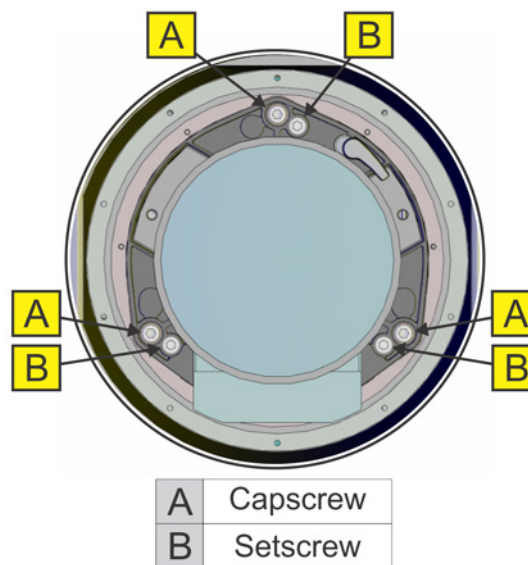
FIGURE 2-4 SCREW LOCATIONS
