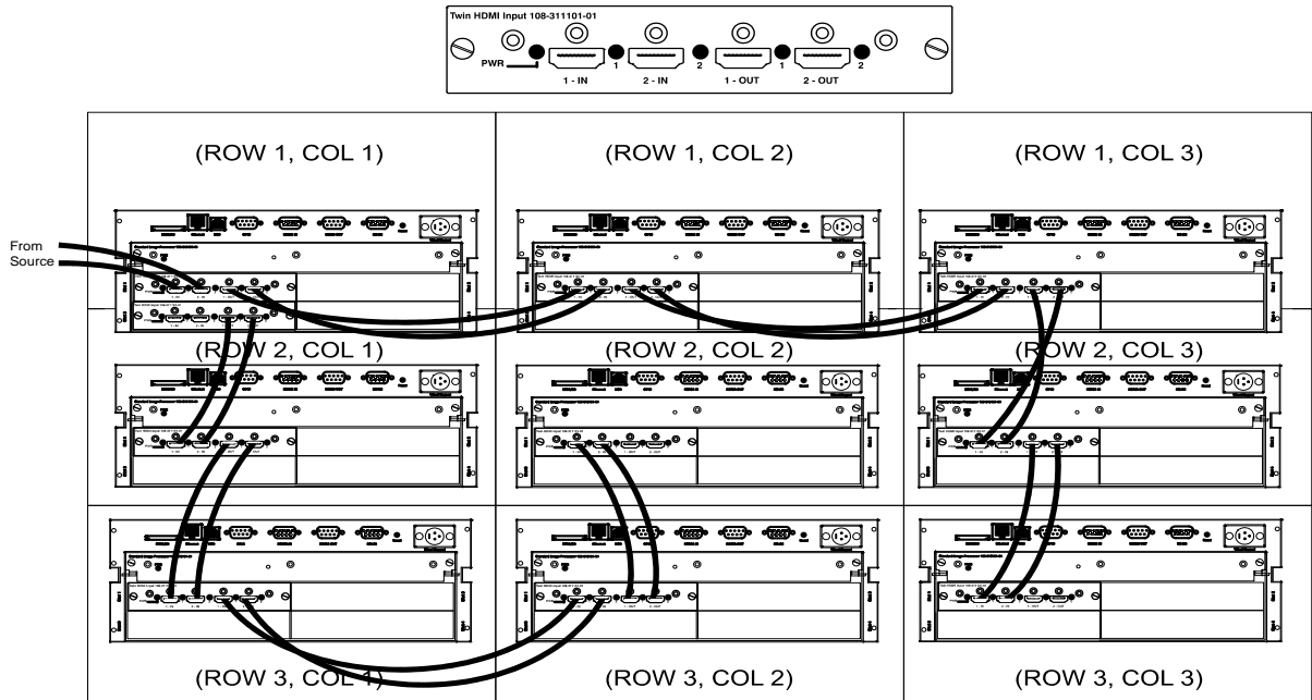
FIGURE 2-10 3X3 LOOP-THROUGH WIRING SOLUTION
