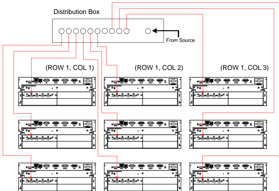
FIGURE 2-5 USE OF DISTRIBUTION BOX
