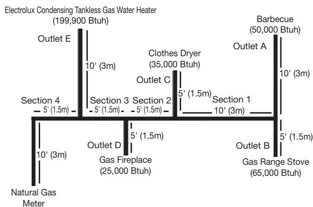
Sample Gas Line
