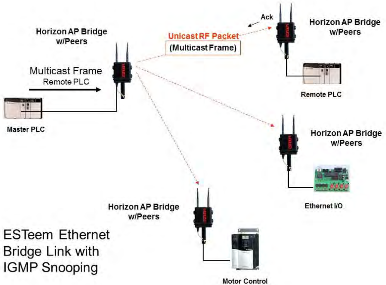
Figure 11: Repeater Peer with IGMP Enabled
