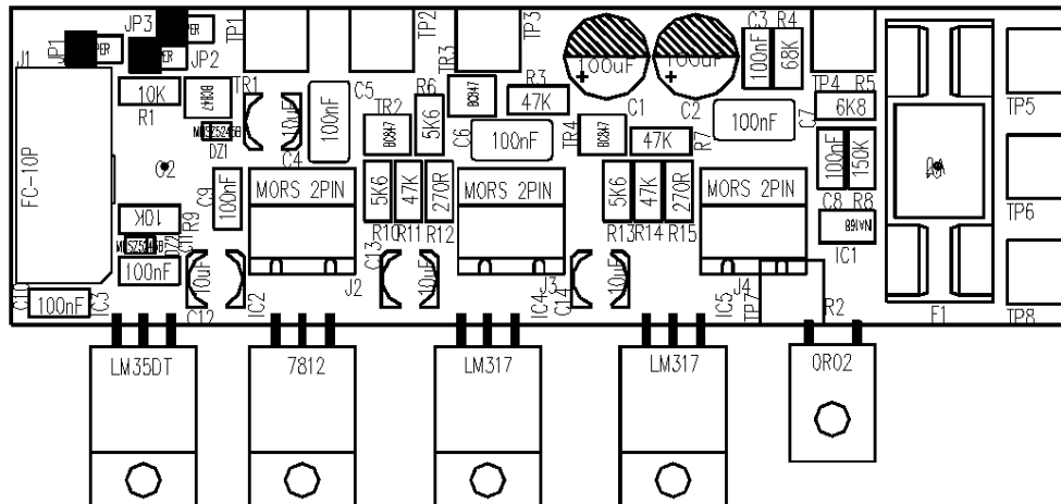
Component layout SCH0300AR0
