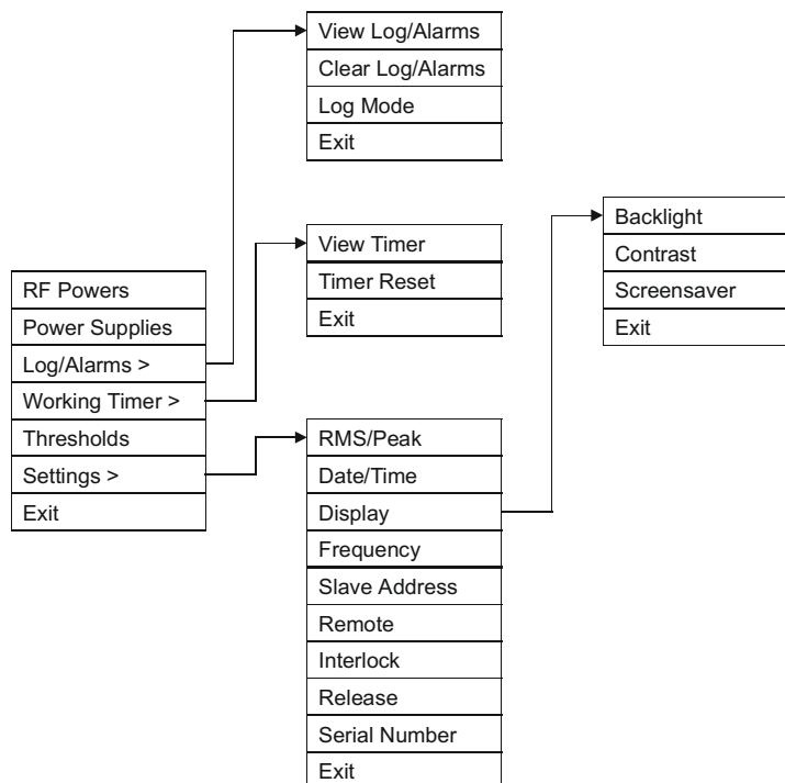
Figure 5: Hierarchical menu structure
