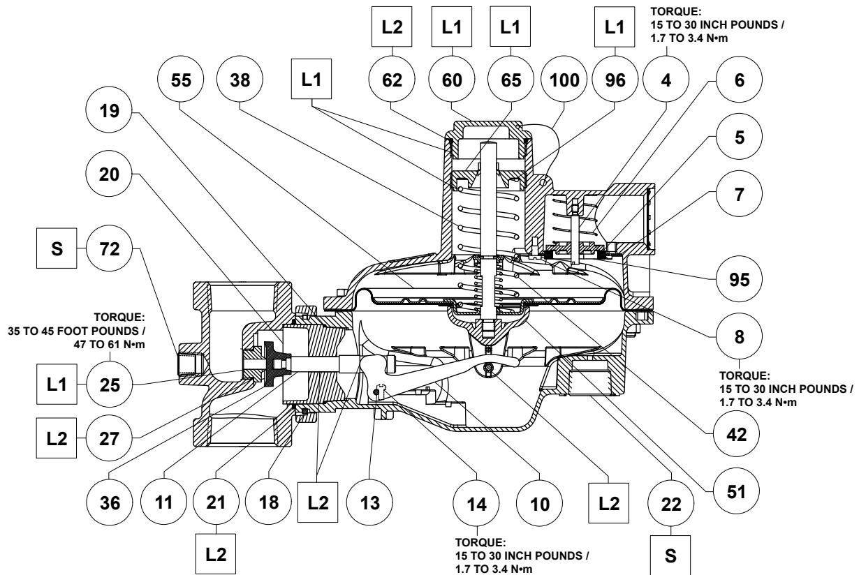
MAIN VALVE
