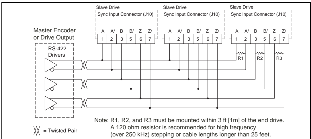
Figure 42: Master/Slave Encoder Connections
