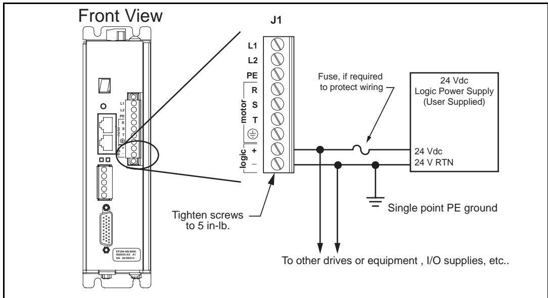
Figure 19: Logic Power Supply Wiring Diagram
