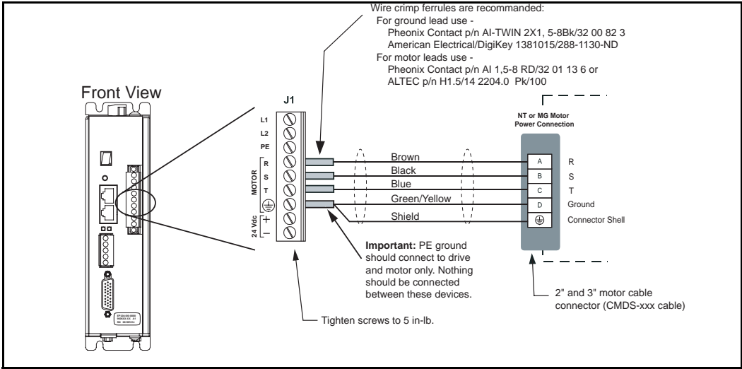
Figure 16: Epsilon EP - NT/MG Motor Power Wiring Diagram
