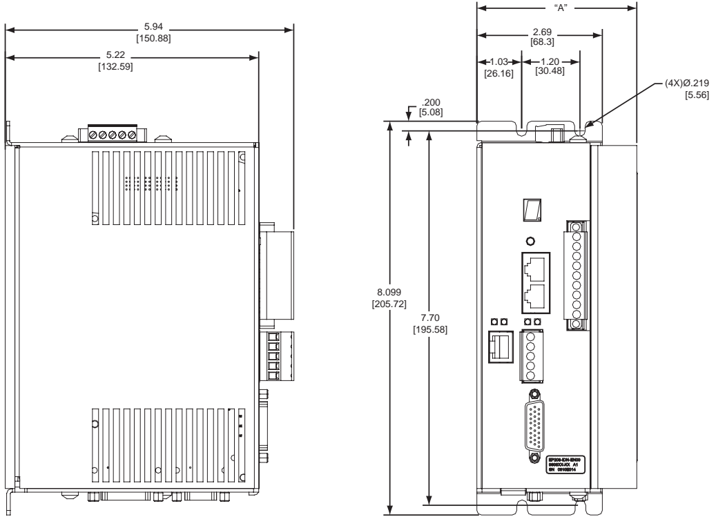
Figure 5: Mechanical Drawing for Epsilon Programming Drive
