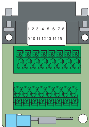
Figure 48: STI-SNCOA Drive Analog/Sync Output Breakout Board
