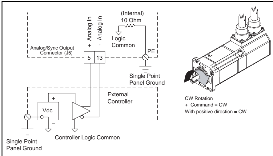
Figure 33: Analog Command, Differential Wiring Diagram
