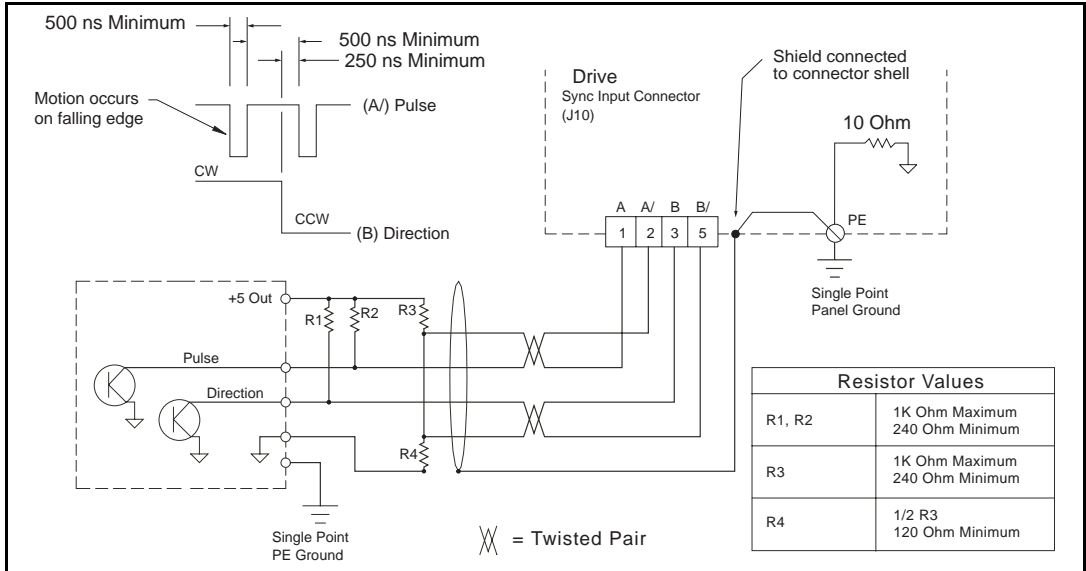
Figure 38: Pulse Mode, Single Ended Output to Differential Input
