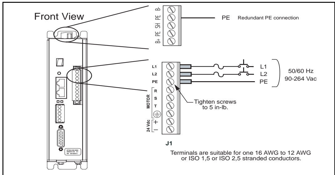
Figure 14: Epsilon EP AC Power Wiring Diagram
