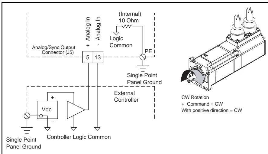
Figure 34: Analog Command, Single Ended Wiring Diagram
