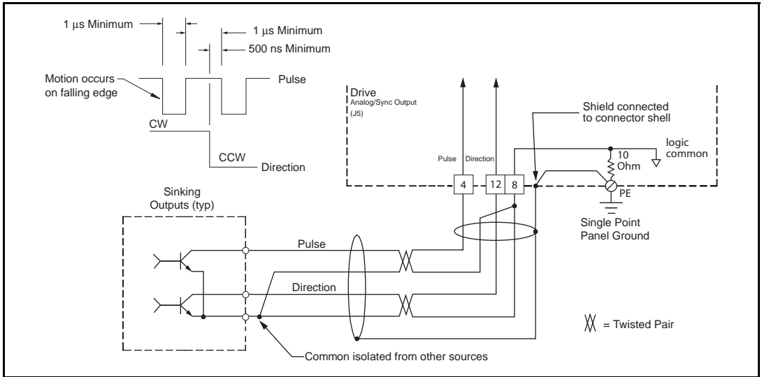
Figure 39: Pulse Mode, Single Ended Output to Single Ended Input (twisted pair cable)
