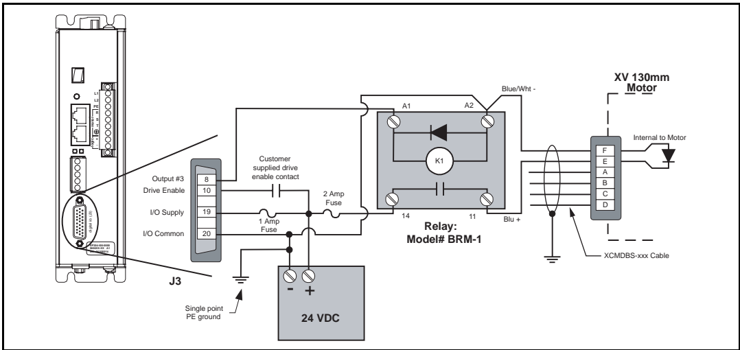
Figure 25: Epsilon EP/XV 130 mm Motor Brake Wiring Diagram using the I/O Connector
