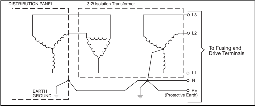
Figure 10: Three-Phase WYE (ungrounded) Distribution to a Three-Phase Delta/WYE Isolation Transformer
