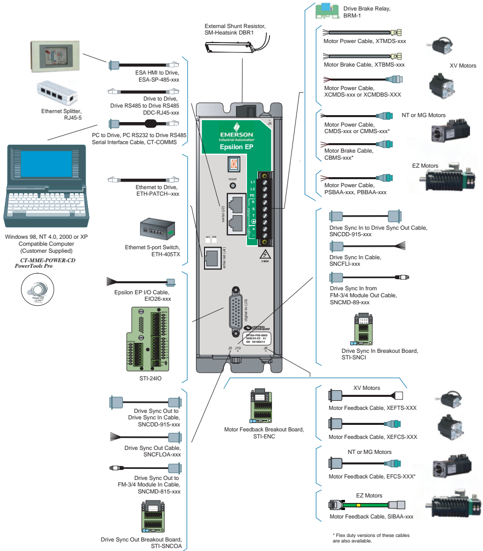
Figure 46: Epsilon EP-P Drive shown with Options
