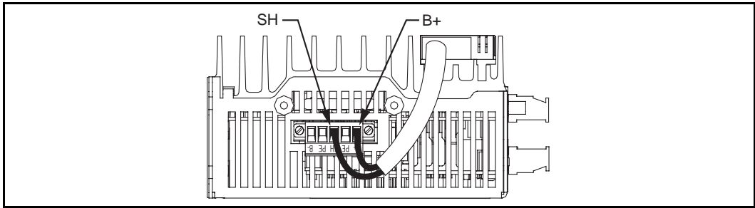
Figure 15: Shunt Resistor Connections showing SM-Heatsink DBR-1 Kit
