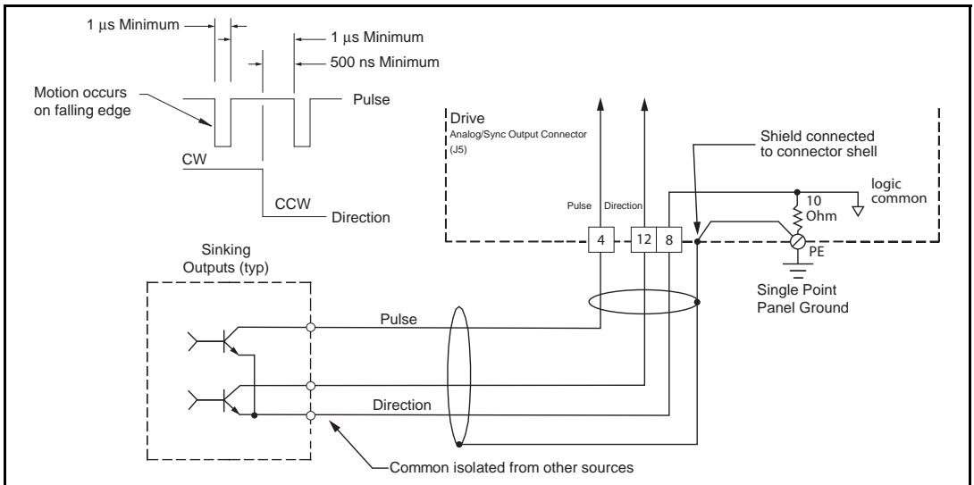
Figure 40: Pulse Mode, Single Ended Output to Single Ended Input (non-twisted pair cable)
