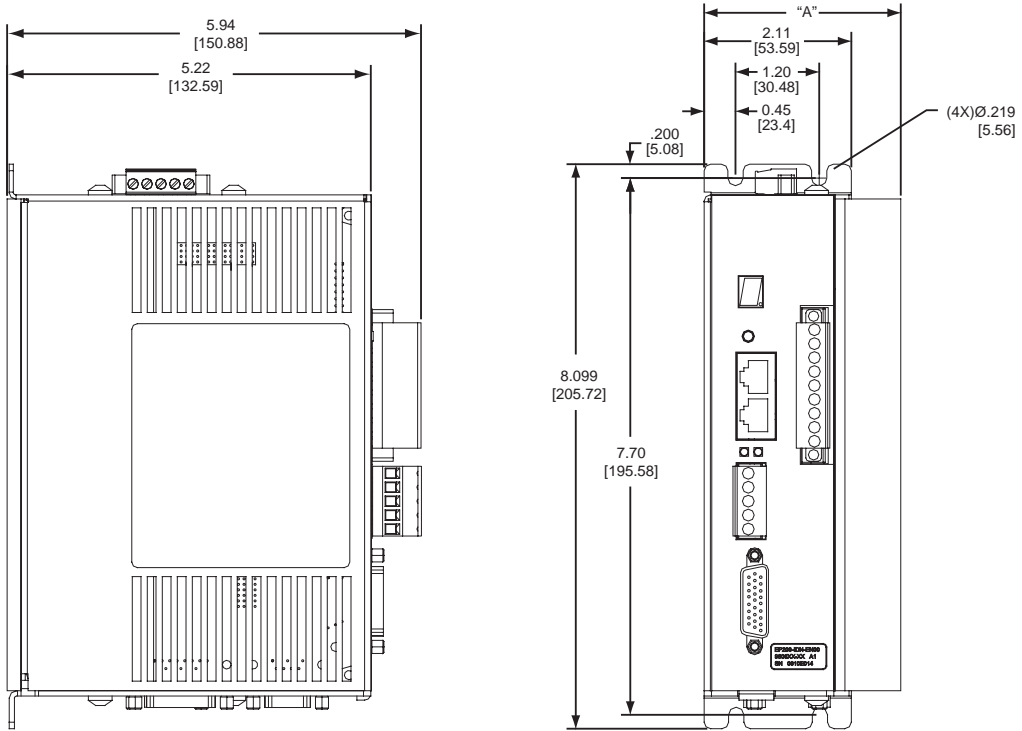
Figure 4: Mechanical Drawing for Epsilon Base and Indexing Drives
