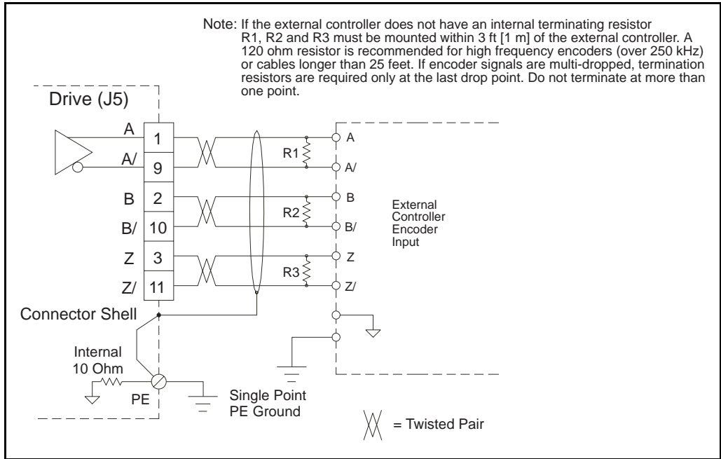
Figure 35: Analog/Sync Output Connector (J5) Encoder Output Wiring
