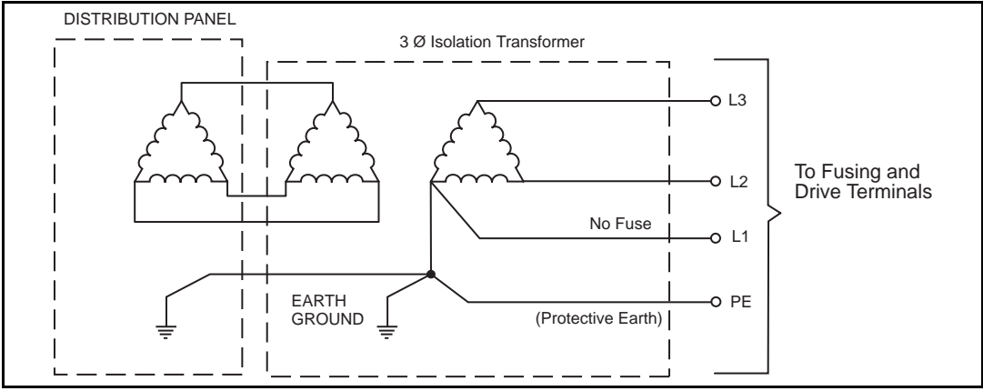
Figure 11: Three-Phase Delta (ungrounded) Distribution to a Three-Phase Delta Isolation Transformer
