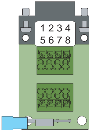
Figure 49: STI-SNCI Drive Sync In Breakout Board
