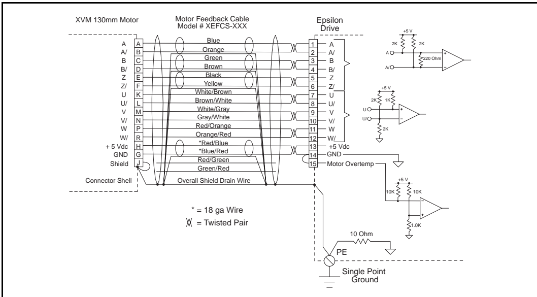
Figure 22: Motor Encoder Feedback Connection For XV 130 mm Motors
