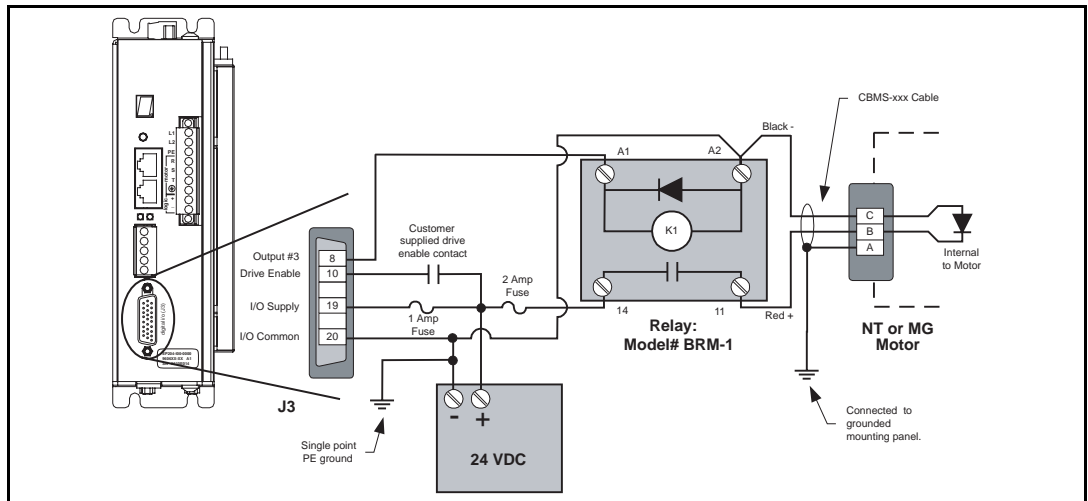
Figure 23: Epsilon EP to NT or MG Motor Brake Wiring Diagram
