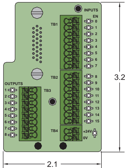
Figure 47: Dimensions of the STI-24IO Board
