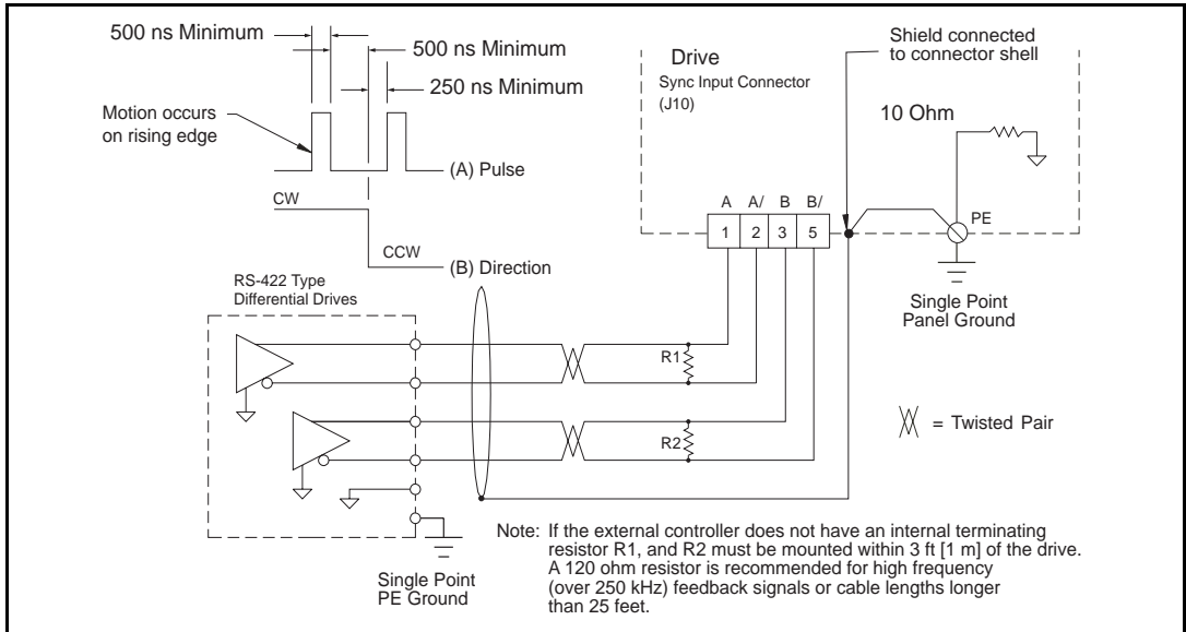
Figure 37: Pulse Mode, Differential Output to Differential Input
