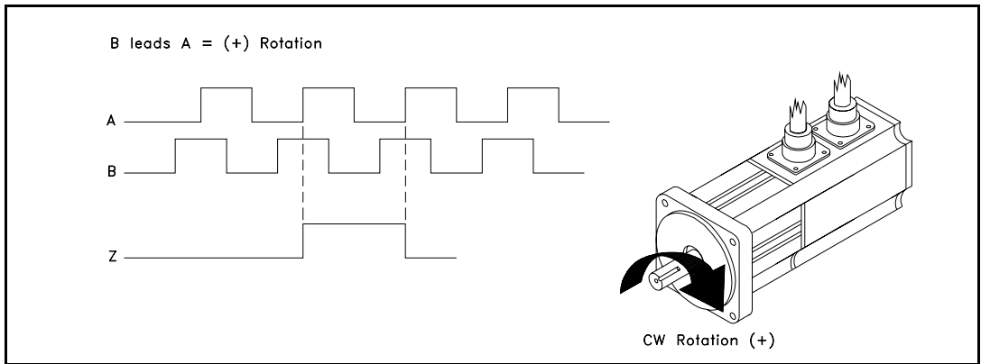
Figure 36: Direction Convention Diagram
