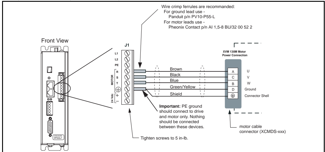
Figure 18: Epsilon EP - XV 130 mm Motor Power Wiring Diagram
