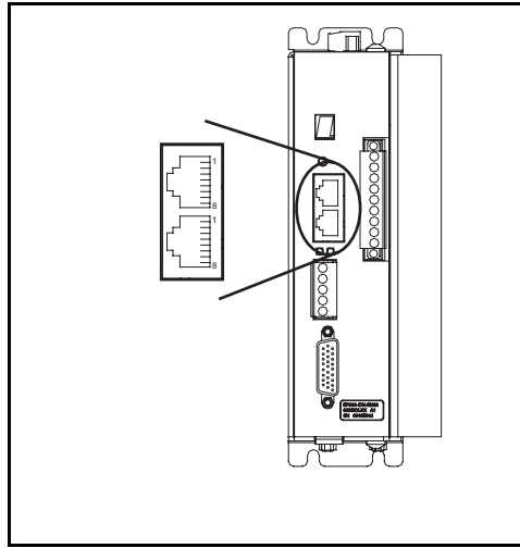
Figure 43: Epsilon EP Serial Communication Connector
