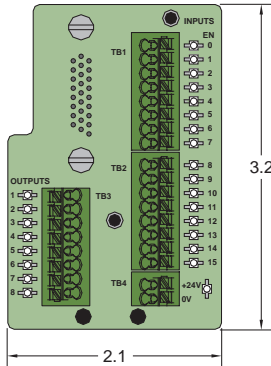
Figure 28: STI-24IO Interface Board
