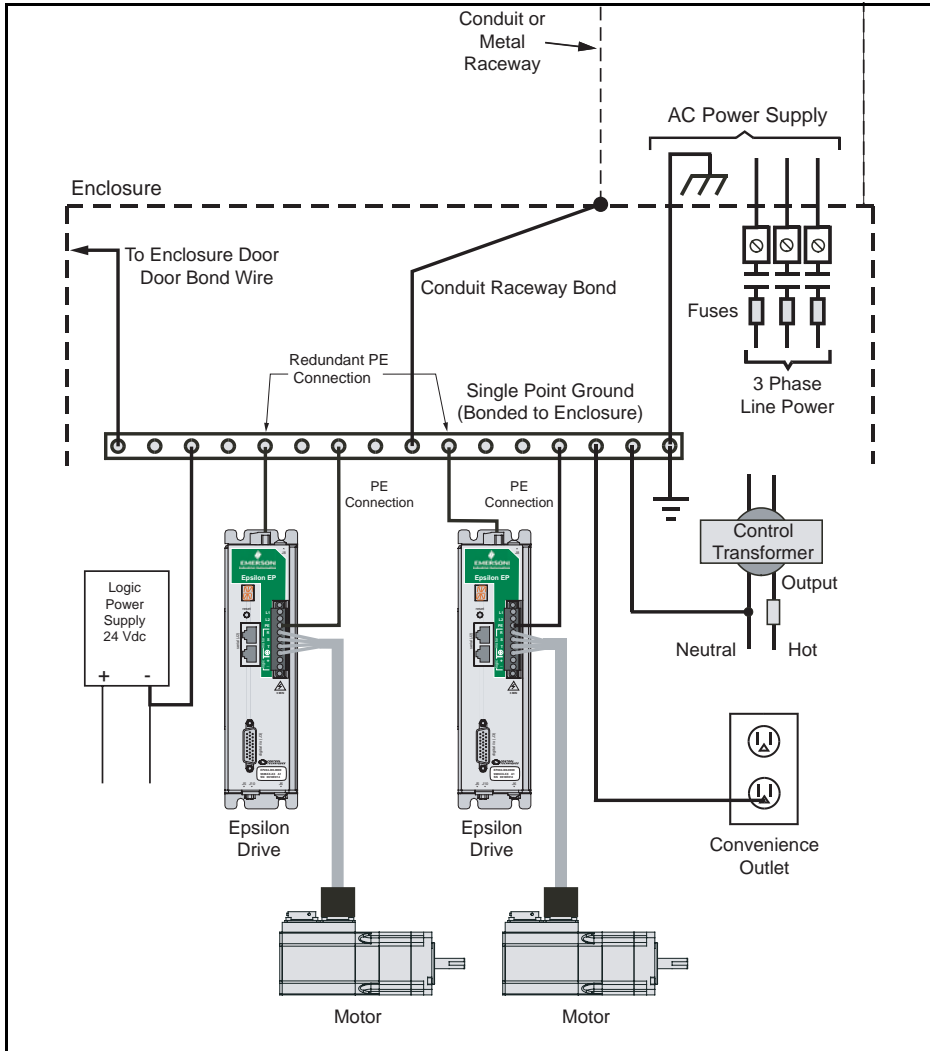
Figure 6: Typical System Grounding Diagram
