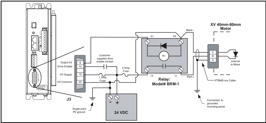
Figure 24: Epsilon EP/XV 40-80 mm Motor Brake Wiring Diagram
