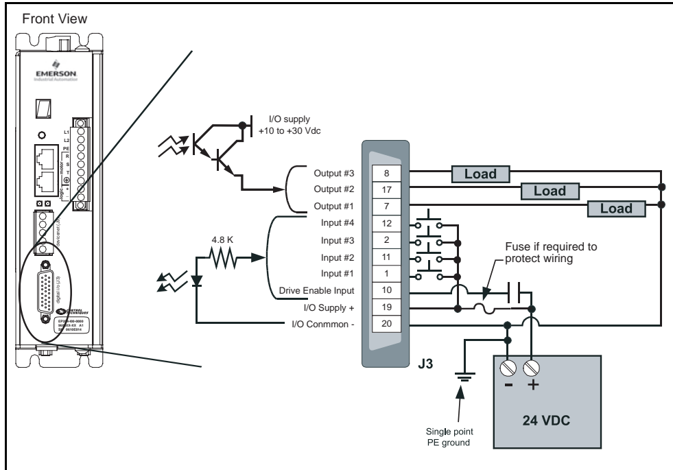
Figure 26: Epsilon EP-B Input/Output Wiring Diagram
