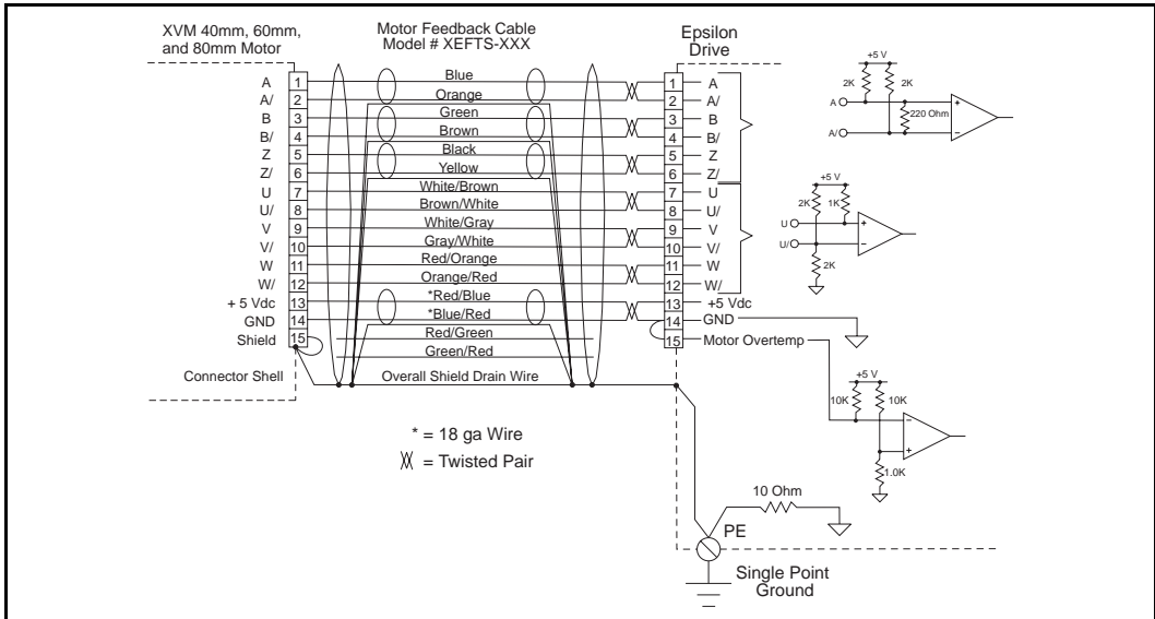
Figure 21: Motor Encoder Feedback Connection For XV 40-80 mm Motors
