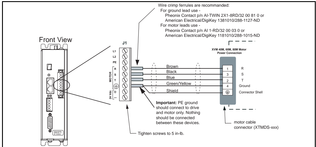
Figure 17: Epsilon EP - XV 40 mm - 80 mm Motor Power Wiring Diagram
