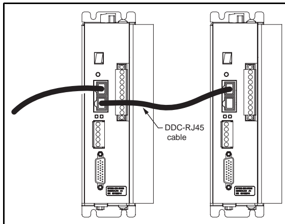
Figure 44: 2 Epsilon Drives Daisy Chained Together
