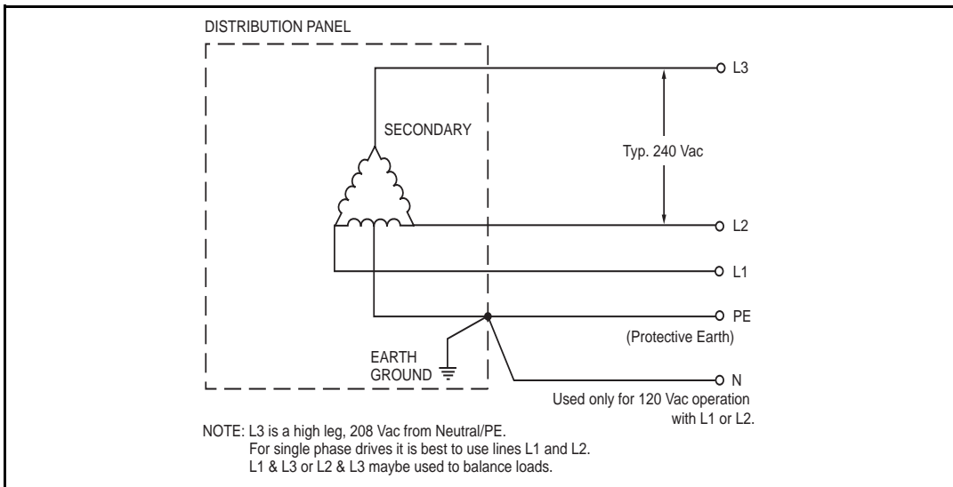
Figure 9: Three Phase Delta (with mid-phase GND) Distribution, 120 Vac split/240 Vac 3Ø supply
