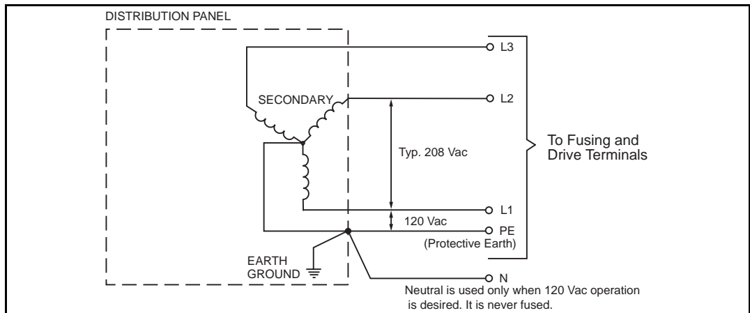
Figure 7: Earth Grounded WYE Distribution Transformer, 120/208Y 3Ø
