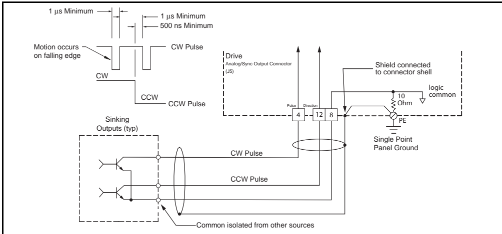
Figure 41: Pulse/Pulse Mode, Single Ended Output to Single Ended Input (non-twisted pair cable)
