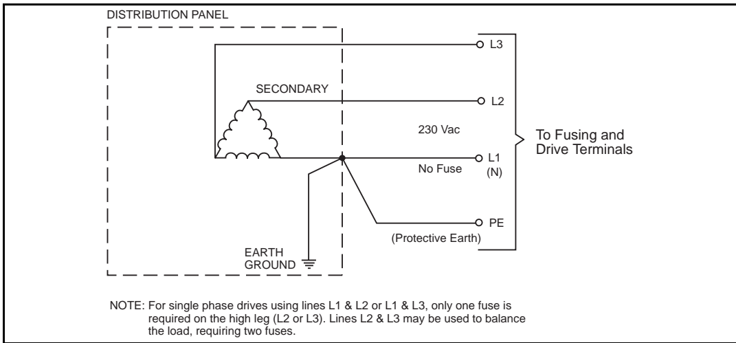
Figure 8: Earth Grounded Delta Distribution Transformer, 240 Vac 3Ø
