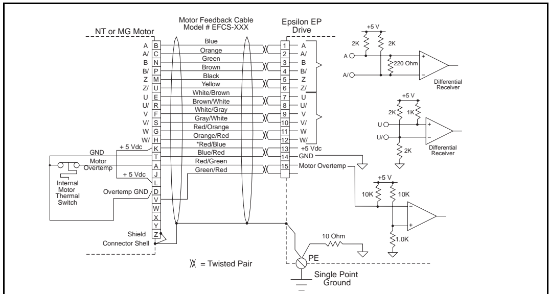
Figure 20: Motor Encoder Feedback Connector Pinout
