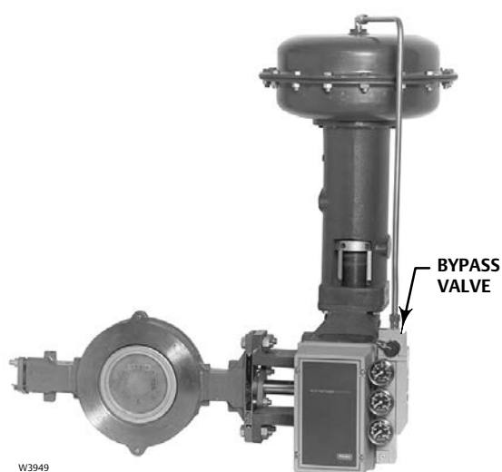
FISHER 3610J PNEUMATIC POSITIONER WITH 1052 ACTUATOR AND ECCENTRIC DISC VALVE
