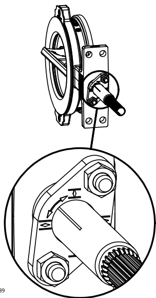
Figure 4. Travel Indication
