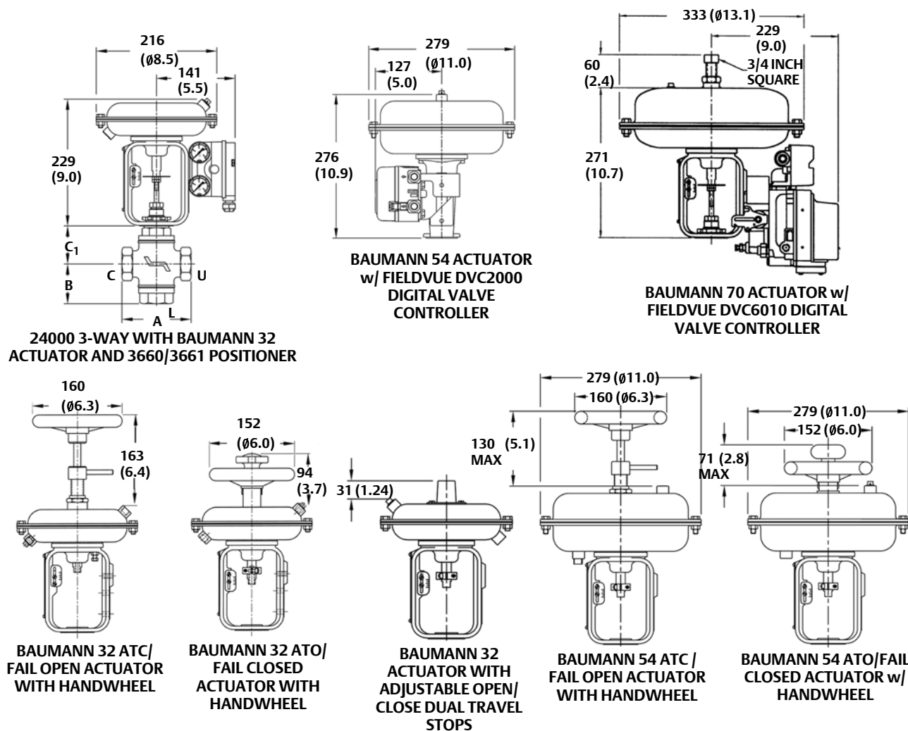
Figure 8. Dimensional Drawings
