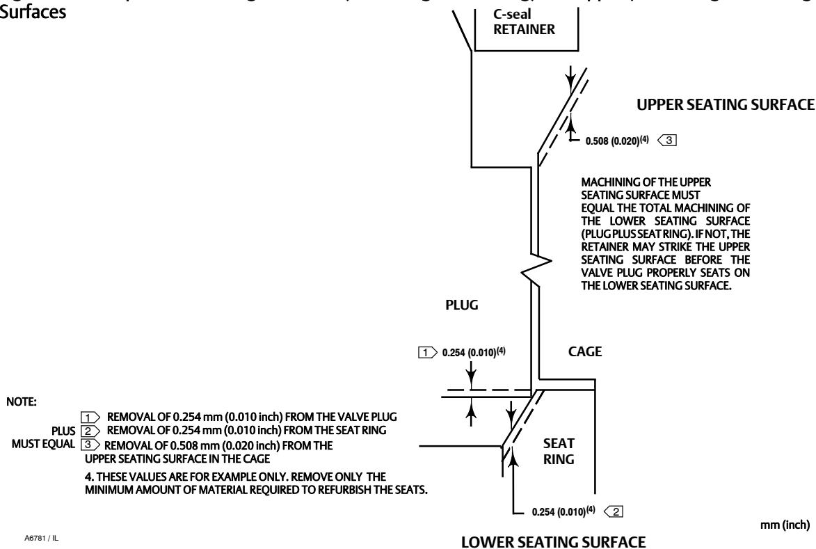
Figure 11. Example of Machining the Lower (Valve Plug to Seat Ring) and Upper (C-seal Plug Seal to Cage) Seating Surfaces
