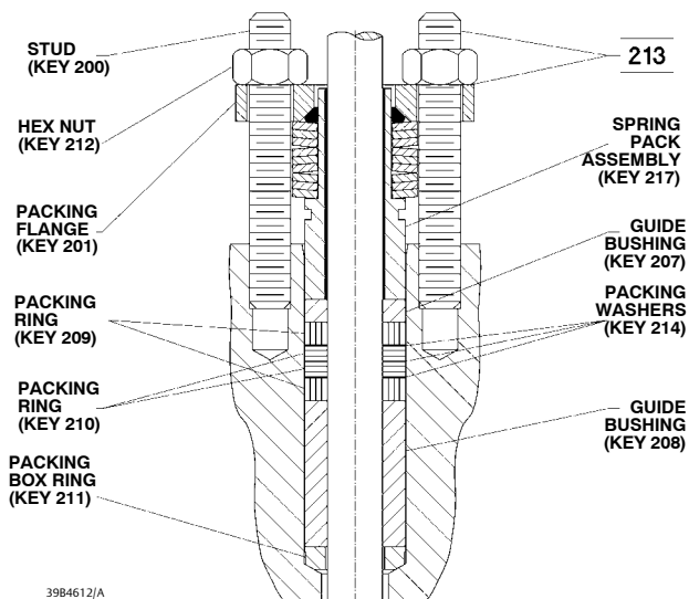
Figure 16. Typical ENVIRO-SEAL Packing System with Graphite ULF Packing
