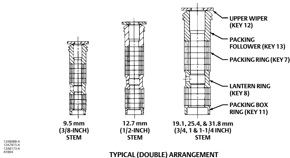
Figure 4. PTFE/Composition Packing Arrangements for Plain or Extension Bonnets
