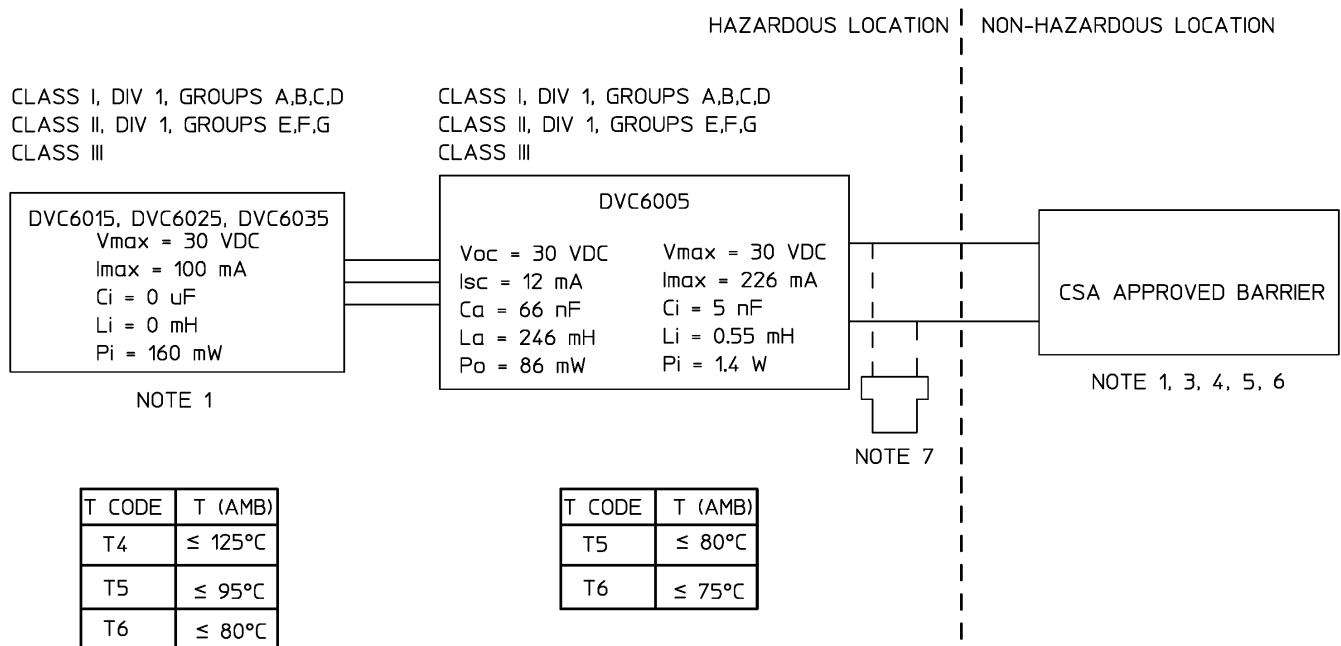
Figure B-3. CSA Schematic for FIELDVUE DVC6005 SIS with DVC6015, DVC6025, and DVC6035
