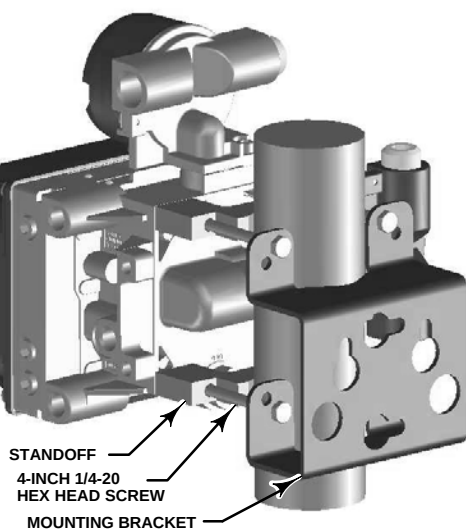
PIPESTAND MOUNTING
