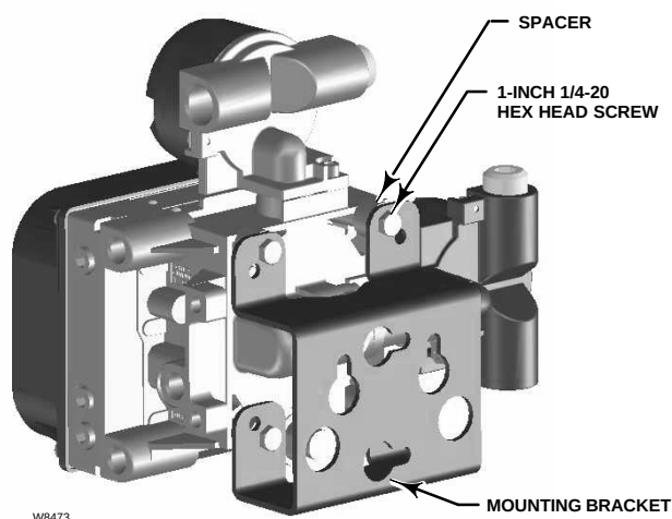
WALL MOUNTING
