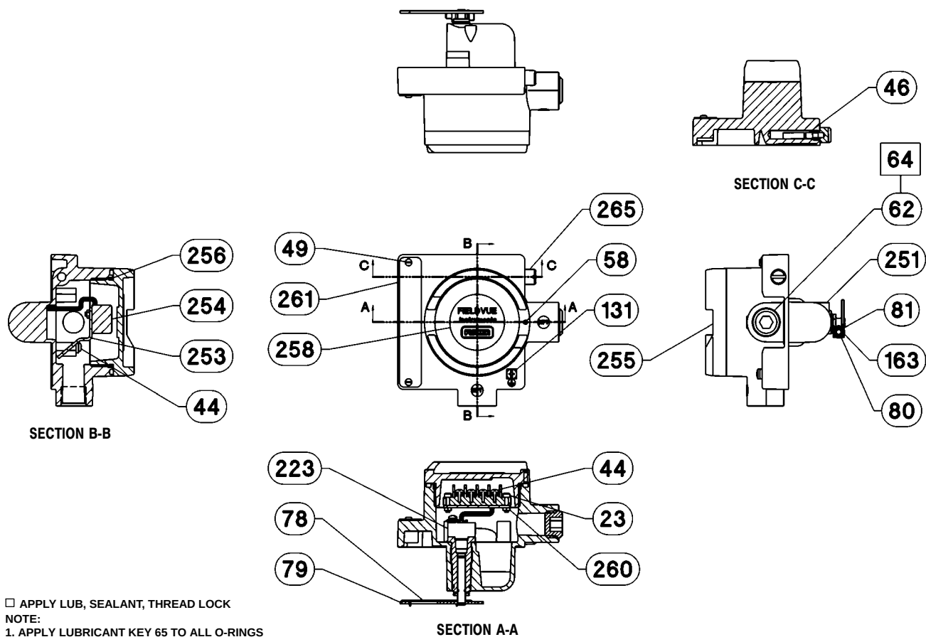
Figure 8-8. FIELDVUE DVC6035 Feedback Unit Assembly
