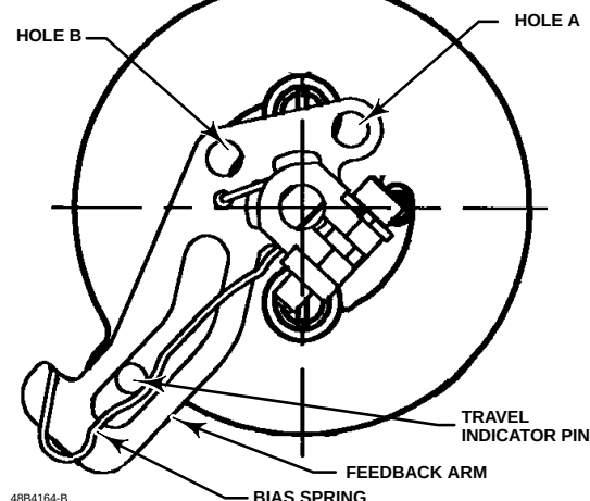
Figure 2-11. Positioning Travel Indicator Pin in the Feedback Arm (Viewed as if Looking from the FIELDVUE DVC6030 SIS toward the Actuator)
