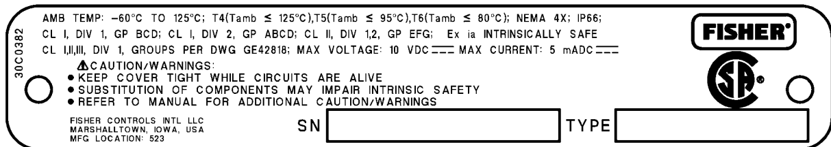
Figure B-5. Typical CSA Nameplates for FIELDVUE DVC6015, DVC6025, and DVC6035
