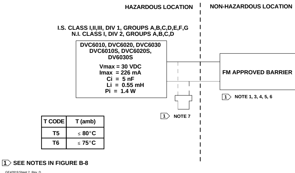
Figure B-6. FM Schematic for FIELDVUE DVC6010 SIS, DVC6020 SIS, and DVC6030 SIS Digital Valve Controllers
