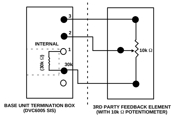
Figure 2-22. Terminal Details for Connecting a FIELDVUE DVC6005 SIS Base Unit and a 10k Ohm External Potentiometer
