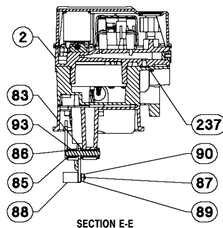
Figure 8-2. FIELDVUE DVC6020 SIS Digital Valve Controller Assembly
