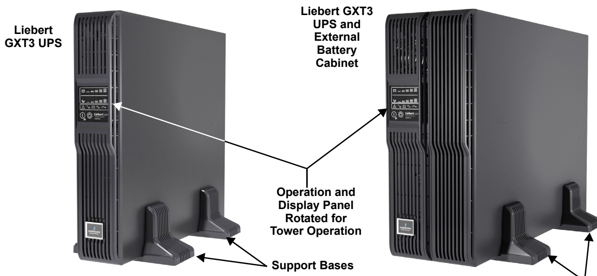
Figure 10 Tower installation
