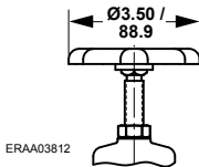
HANDLE DETAIL FOR SIZE 1/2 IN. / DN 15 ONLY
