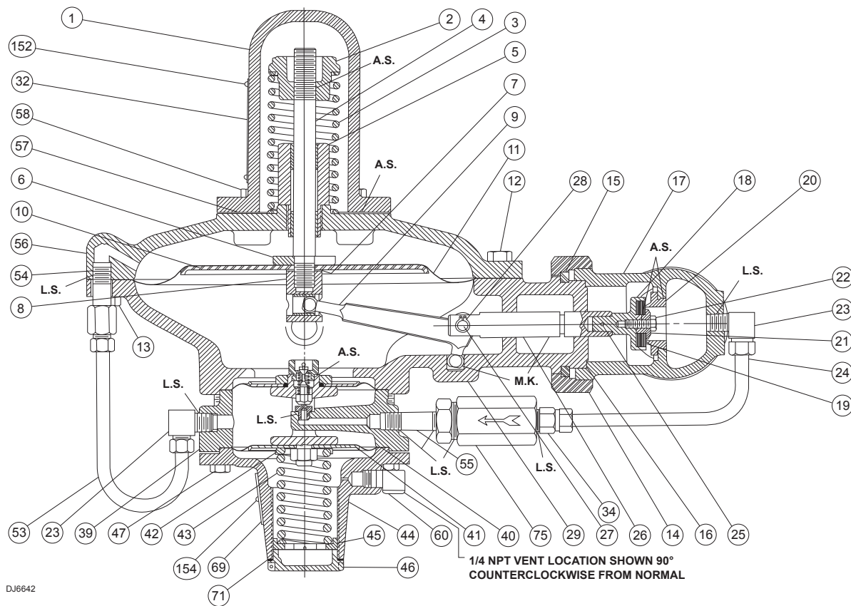
Figure 1. Type 99 Regulator with Low-Pressure Pilot
