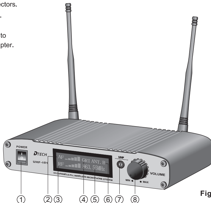
UHF-101 FRONT
