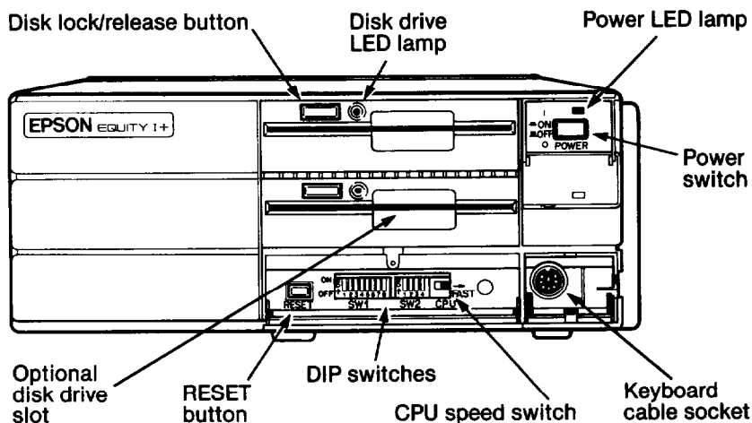
Figure 1-3. Front panel
