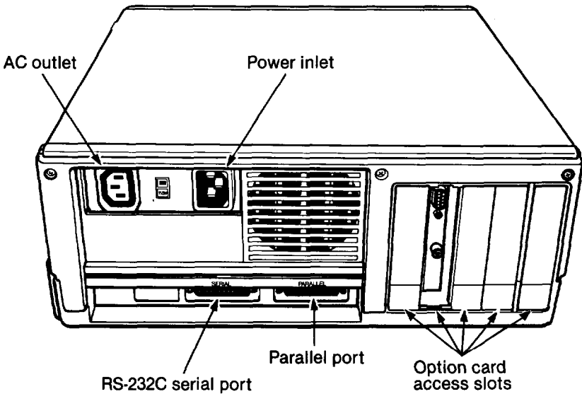
Figure 1-2. Rear panel
