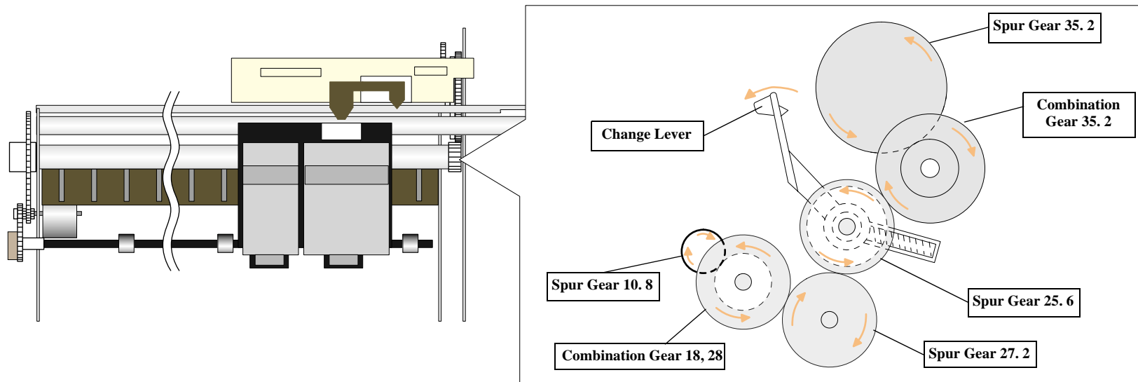
Figure 2-9. Switch the PF motor drive to ASF unit side
