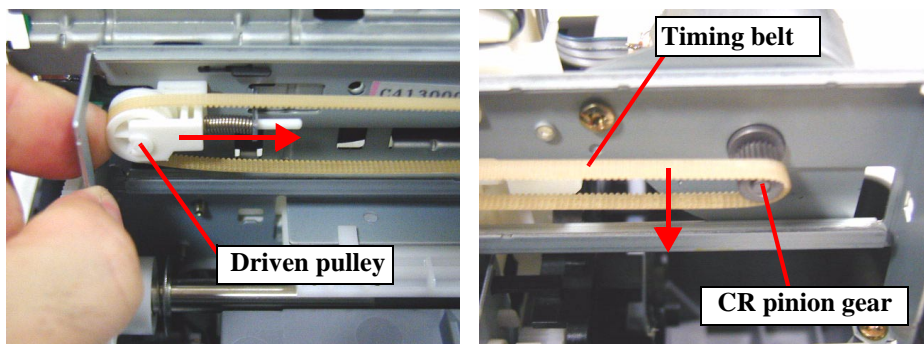
Figure 4-30. Removing the Timing belt
