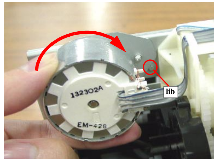
Figure 4-32. Reassembling the CR motor
