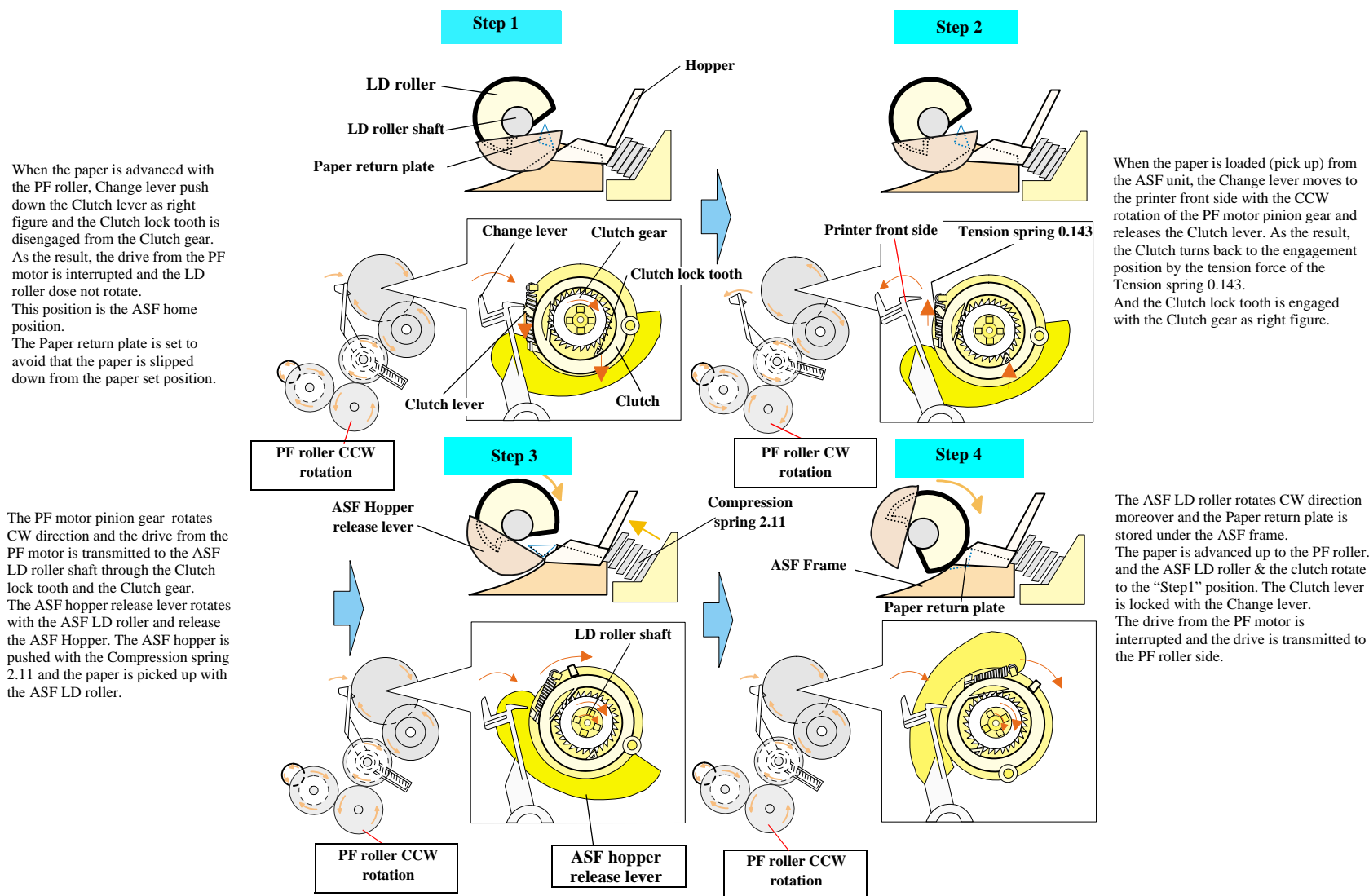
Figure 2-13. ASF Paper Loading Sequence
