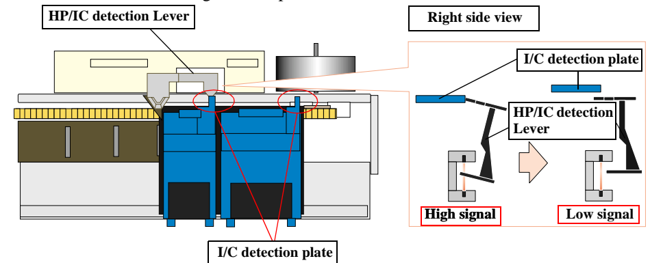
Figure 2-6. I/C detection position
