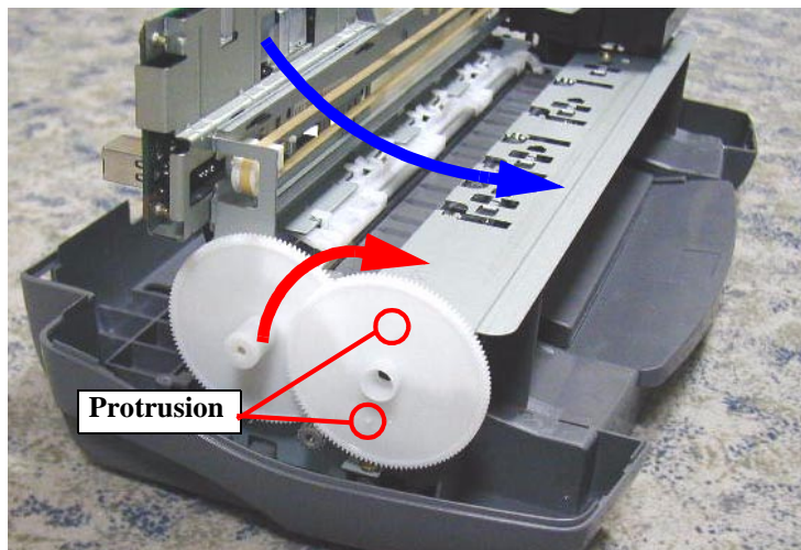
Figure 4-19. Place the OHP sheet
