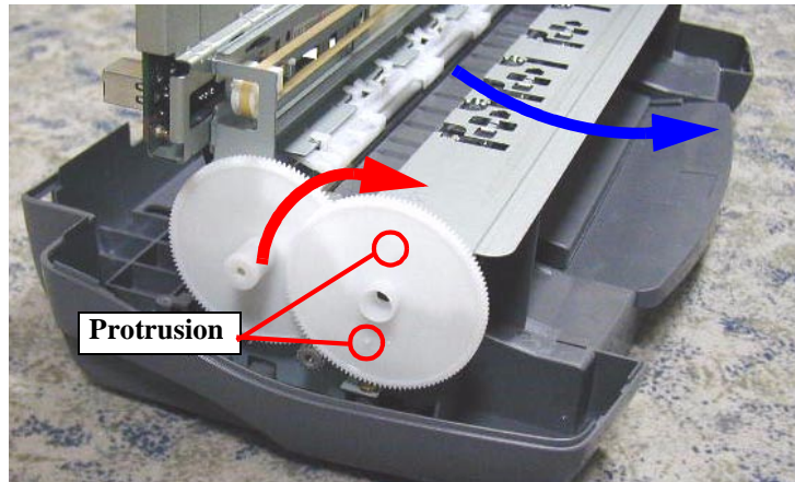
Figure 4-25. Ejecting the OHP sheet
