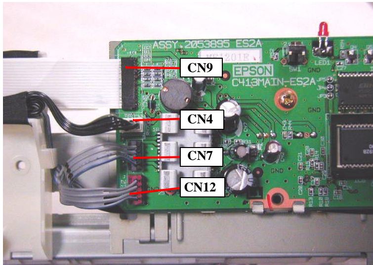
Figure 4-28. Disconnecting the connectors
