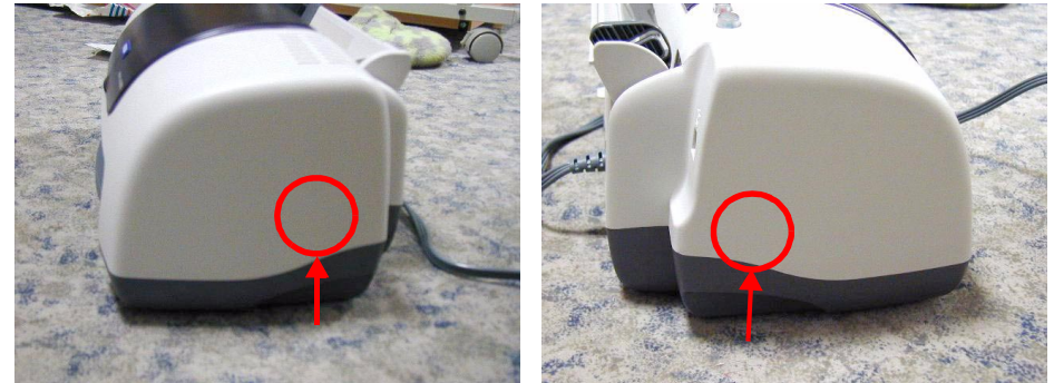
Figure 4-4. Removing the side hook
