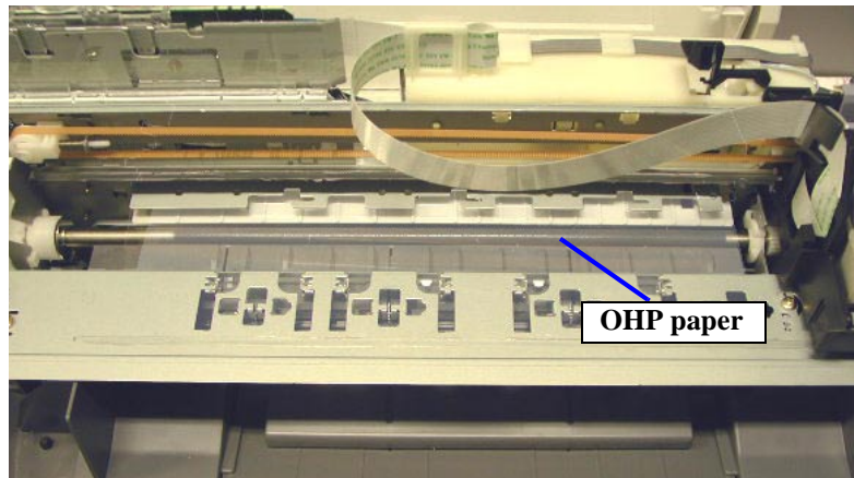
Figure 4-22. Placing the OHP sheet
