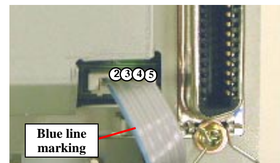
Figure 4-12. Connecting the PS cable(CN2)
