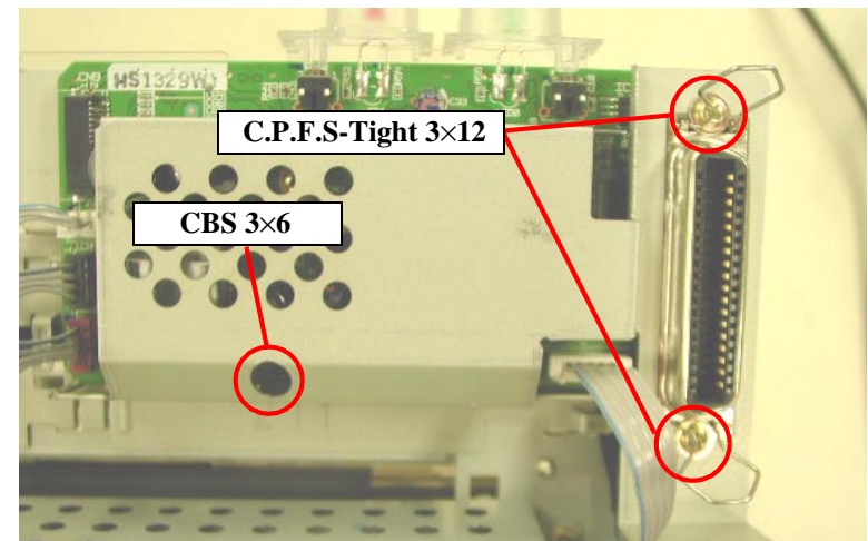
Figure 4-27. Removing the Shield cover
