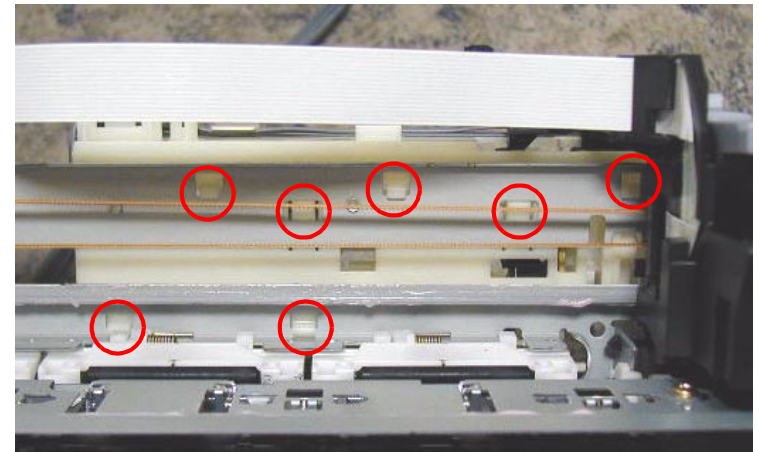
Figure 4-40. Setting seven hooks
