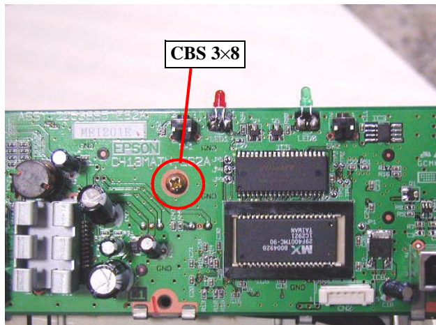
Figure 4-29. Removing the MAIN board
