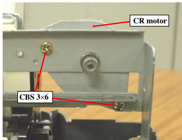
Figure 4-31. Removing the CR motor
