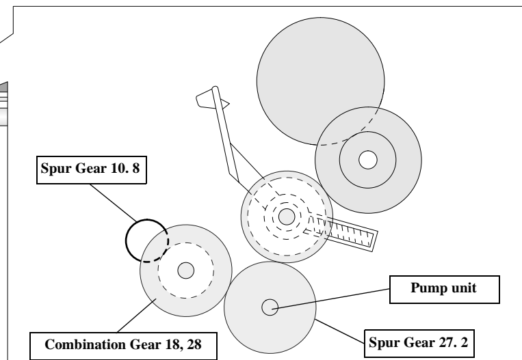
Figure 2-15. PF motor drive transmission path to the Pump unit
