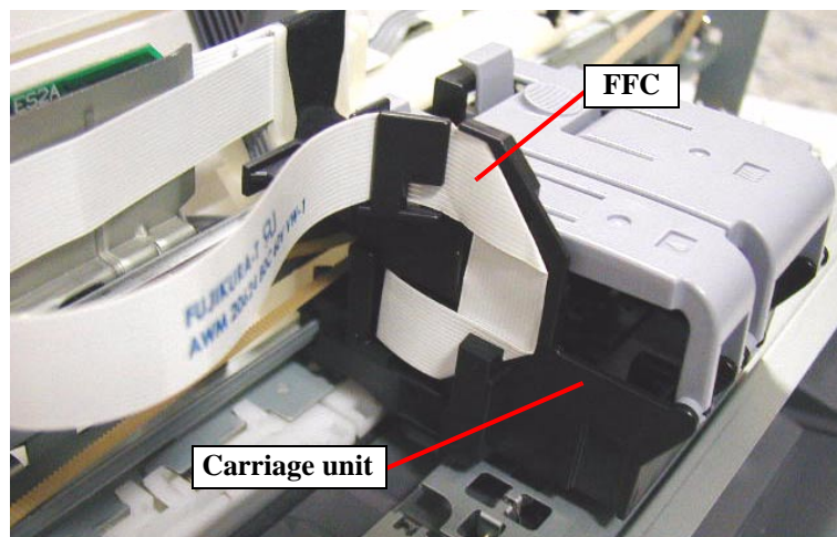
Figure 4-34. Disconnecting the FFC
