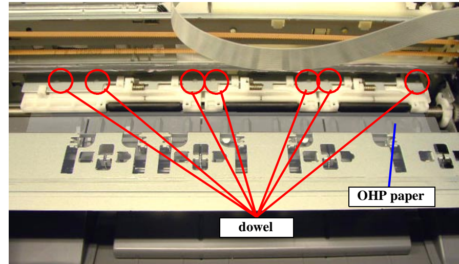
Figure 4-20. Removing the Paper Guide Upper/Left
