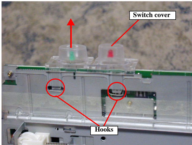
Figure 4-26. Removing the Switch cover
