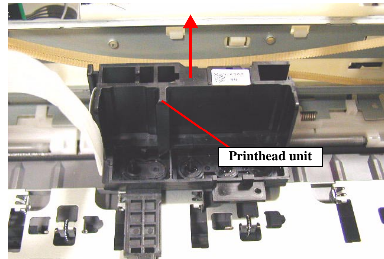
Figure 4-36. Removing the Printhead unit
