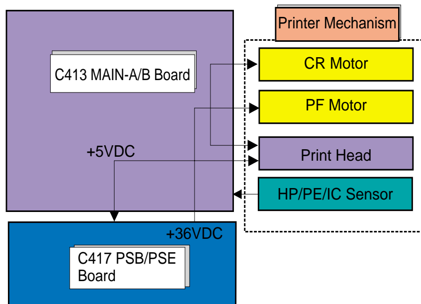
Figure 2-19. Electric Circuit
