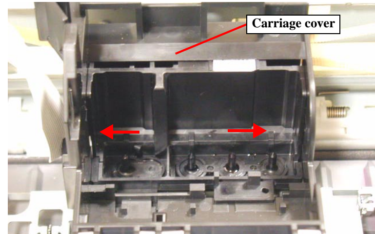
Figure 4-35. Removing the Carriage cover
