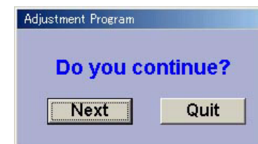
Figure 5-4. Quit function
