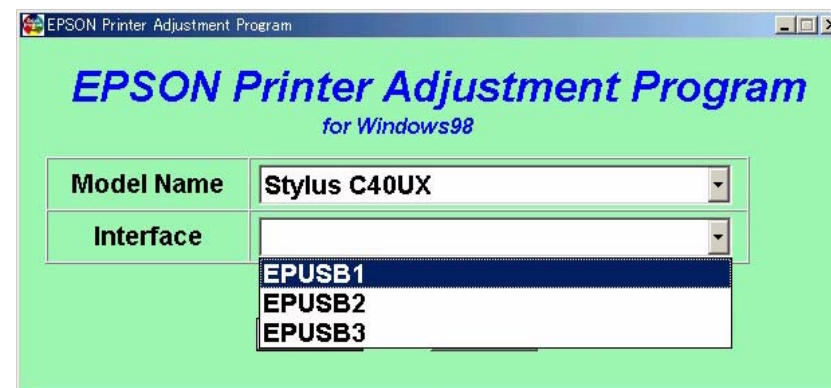
Figure 5-2. Interface Setting
