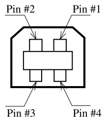
Figure 1-3. USB Pin Assignment
