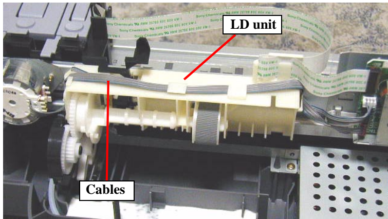
Figure 4-38. Disconnecting the Cables
