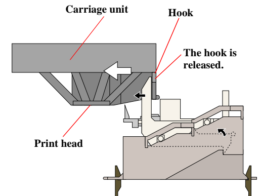
Figure 2-17. Wiper Release
