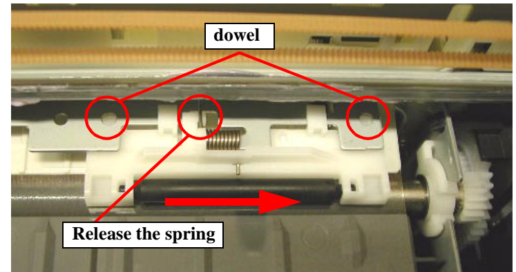
Figure 4-24. Assembling the Paper Guide 2
