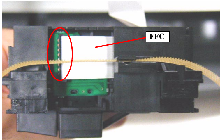
Figure 4-37. Disconnecting the FFC
