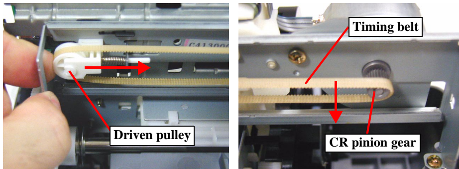
Figure 4-33. Removing the Timing belt
