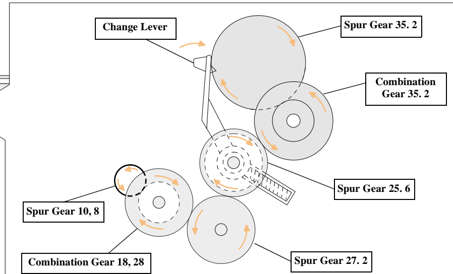
Figure 2-10. PF motor drive transmission path
