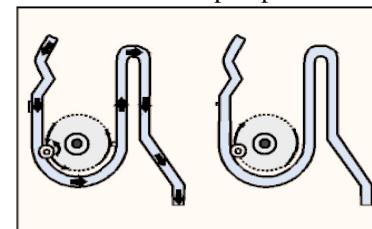
Figure 2-14. Pump mechanism
