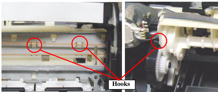
Figure 4-39. Removing the LD unit
