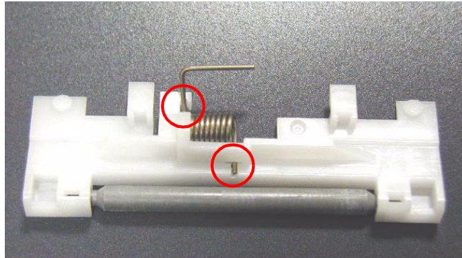
Figure 4-21. Setting the spring to the Paper Guide
