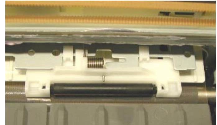
Figure 4-23. Assembling the Paper Guide 1
