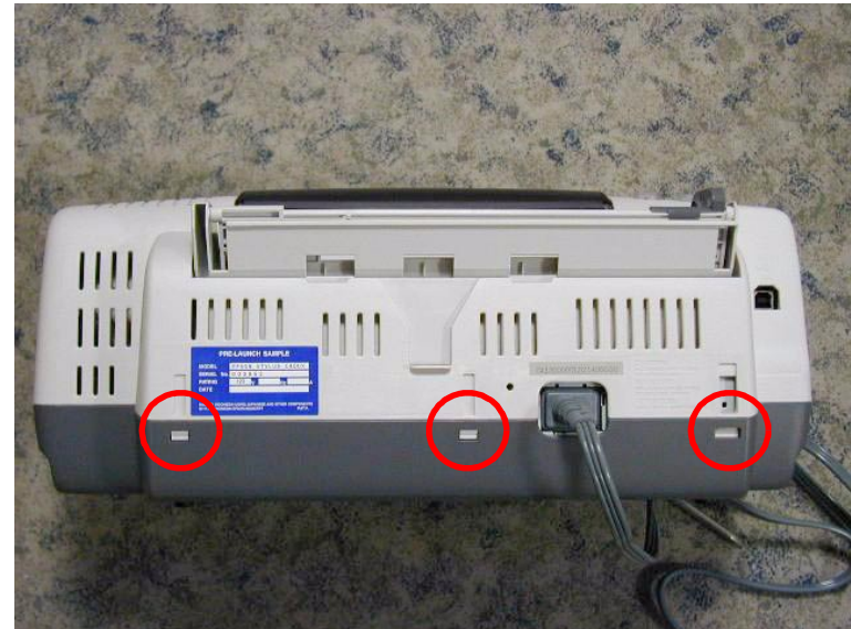
Figure 4-5. Removing the back hook
