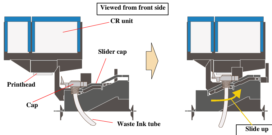
Figure 2-16. Cap Mechanism
