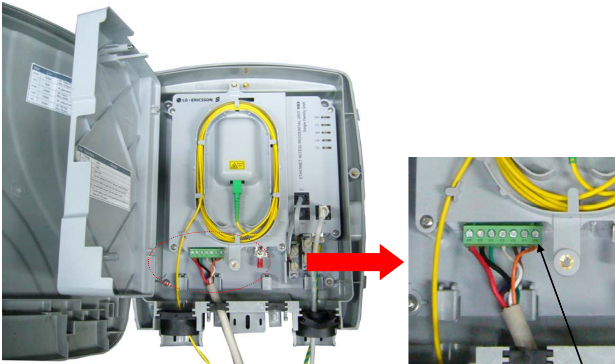
BATTERY INTERFACE
