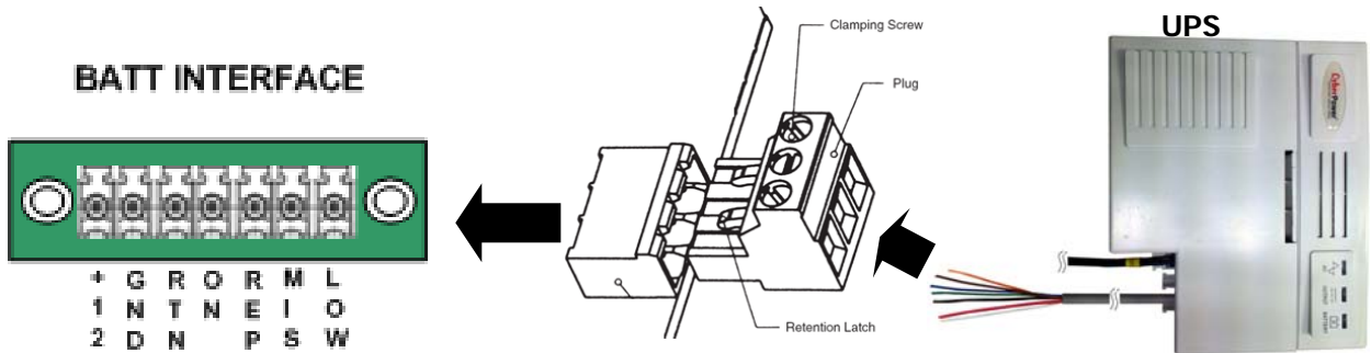
BATTERY INTERFACE
