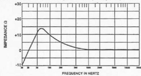
FIGURE 7 — APX-200 Active Equalizer Frequency Response
