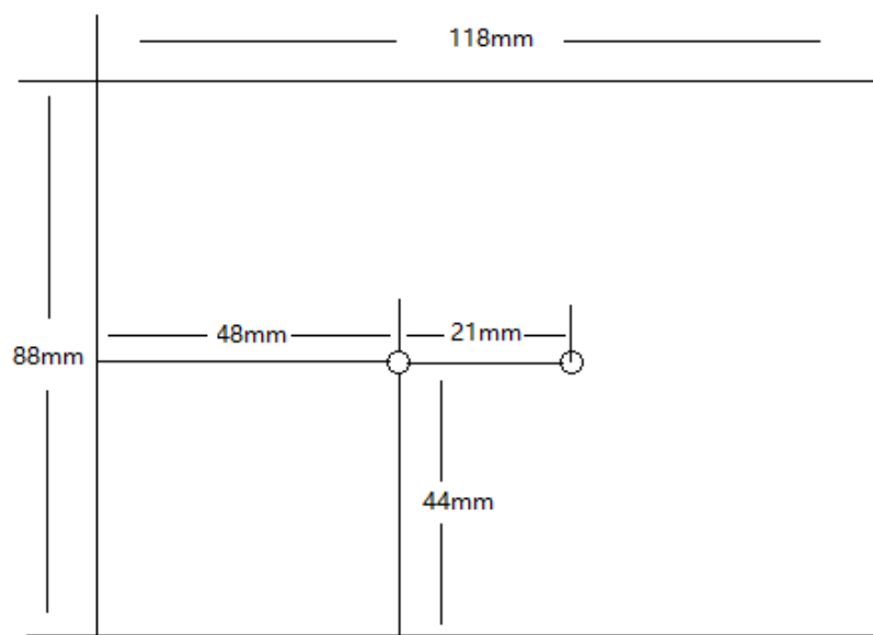
Figure 1-7: ER-600 dimension
