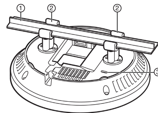
Figure 4 WS-AP3801i Mounted on Drop Ceiling T-bar Rail
