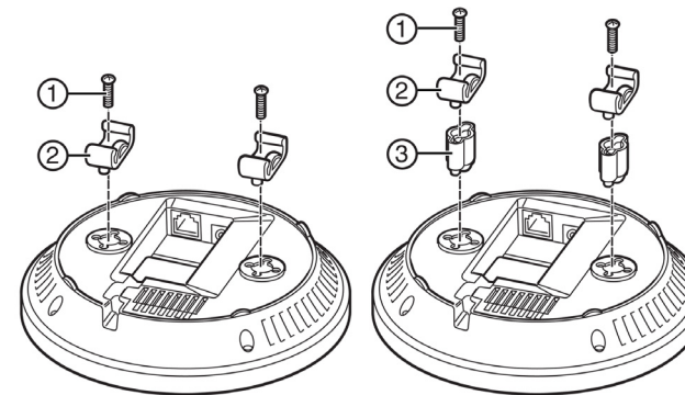
Figure 3 Attaching the T-Rail Connector to the AP
