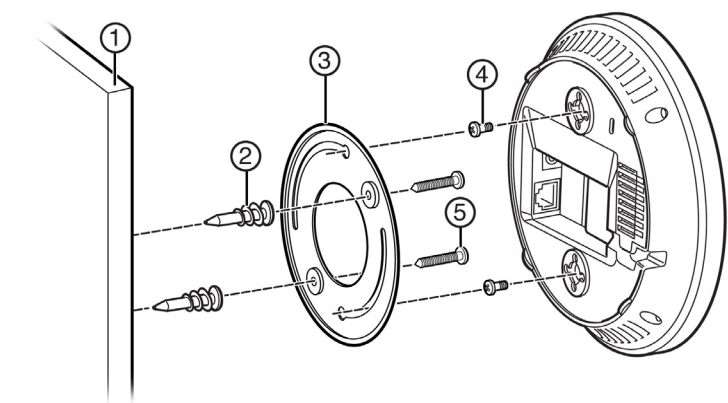
Figure 5 Mounting the WS-AP3801i to a Flat Wall or Solid Ceiling
