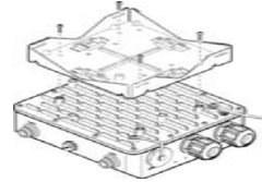
Figure 5 Attaching a Pole Bracket to the AP
