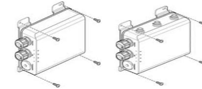
Figure 4 AP7662i and AP7662 Wall Mount "H" Bracket
