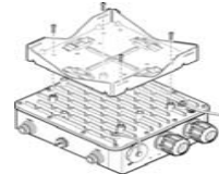
Figure 5 Attaching a Pole Bracket to the AP
