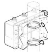
Figure 6 AP with Mounting Bracket—Vertical Pole
