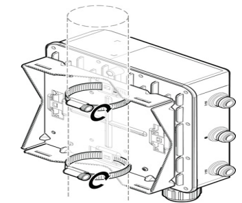
Figure 6 AP with Mounting Bracket—Vertical Pole
