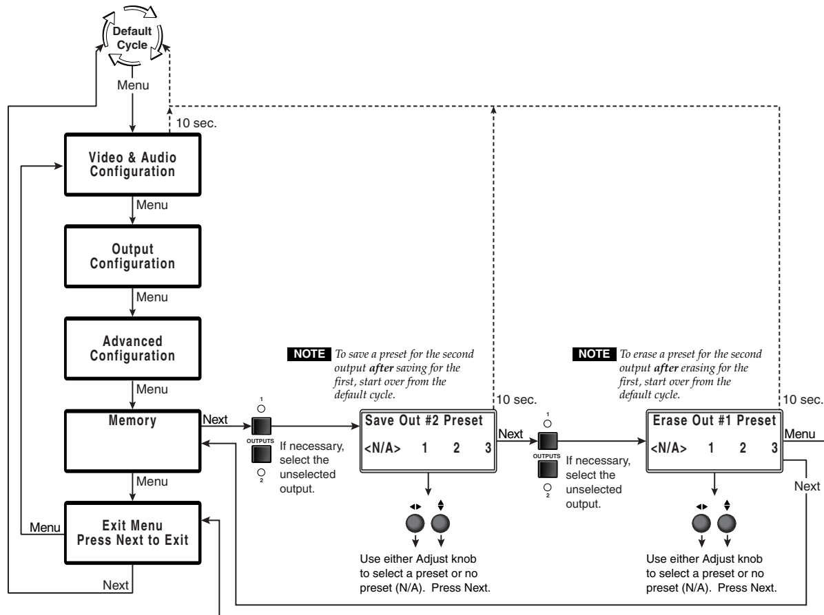
Figure 3-11 — User Presets menu flowchart
