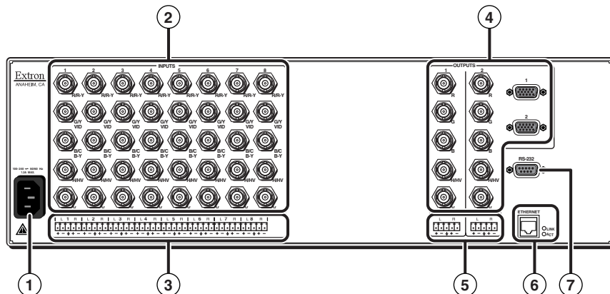
Figure 2-2 — ISM 482 rear panel connectors
