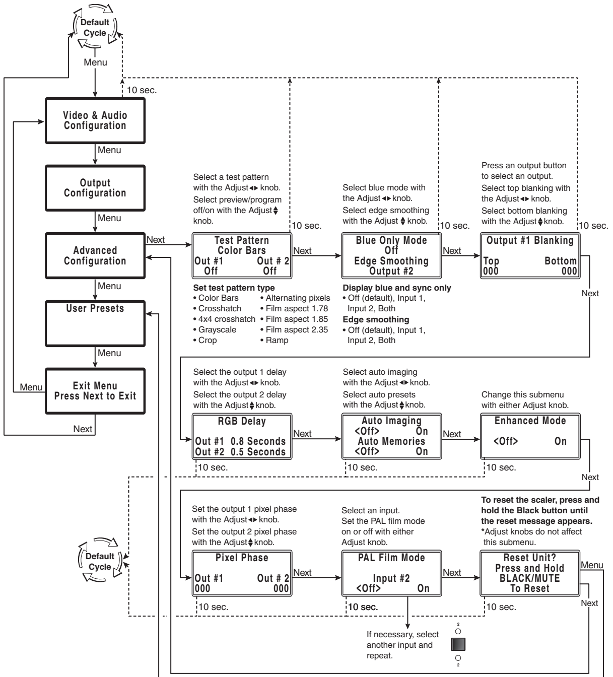
Figure 3-10 — Advanced Configuration menu flowchart
