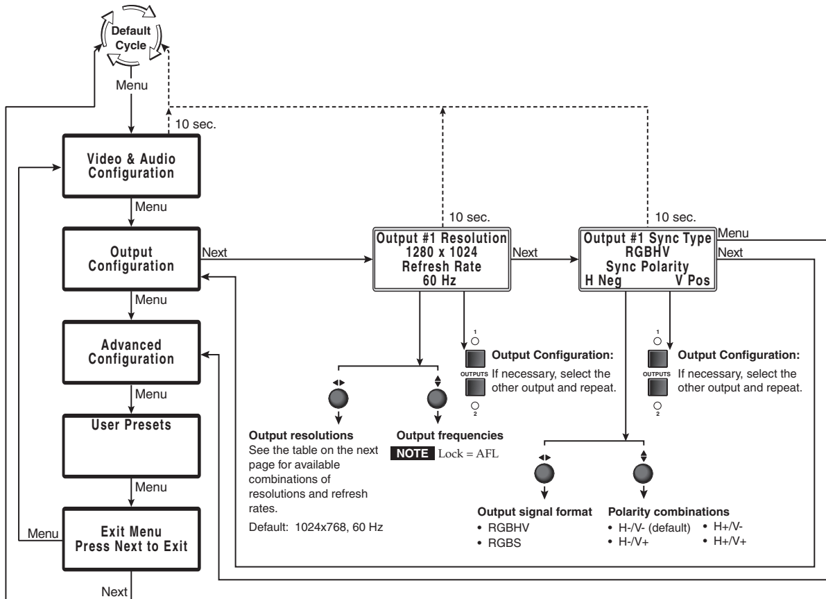
Figure 3-9 — Output Configuration menu flowchart
