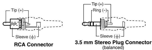
Figure 2-5 — Phono audio connectors
