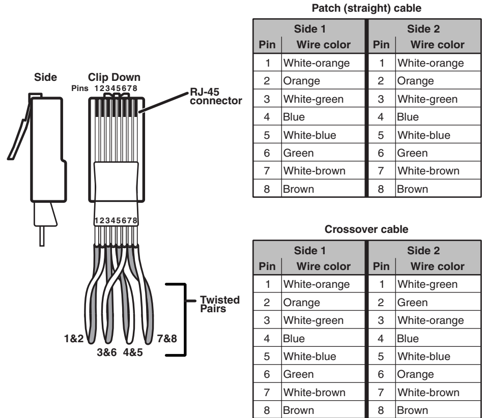
Figure 2-8 — RJ-45 connector pinout tables
