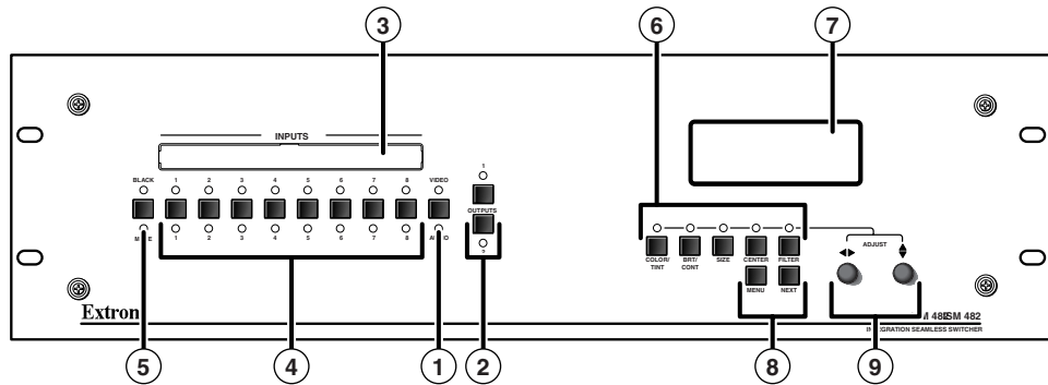
Figure 3-1 — Integration Scaling Matrix Switcher front panel
