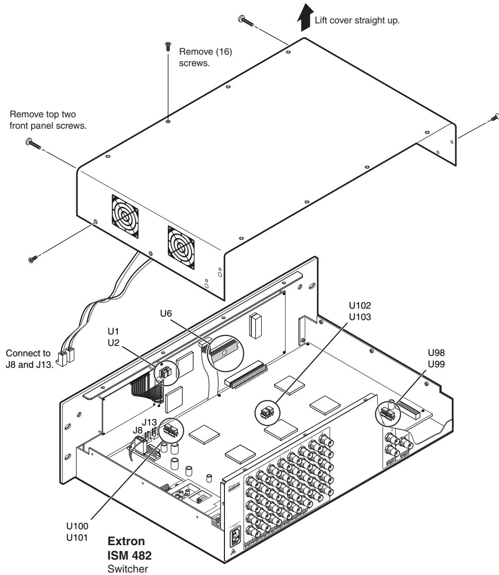
Figure B-1 — Removing the ISM cover
