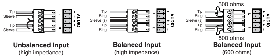
Figure 2-4 — Captive screw connector wiring for inputs
