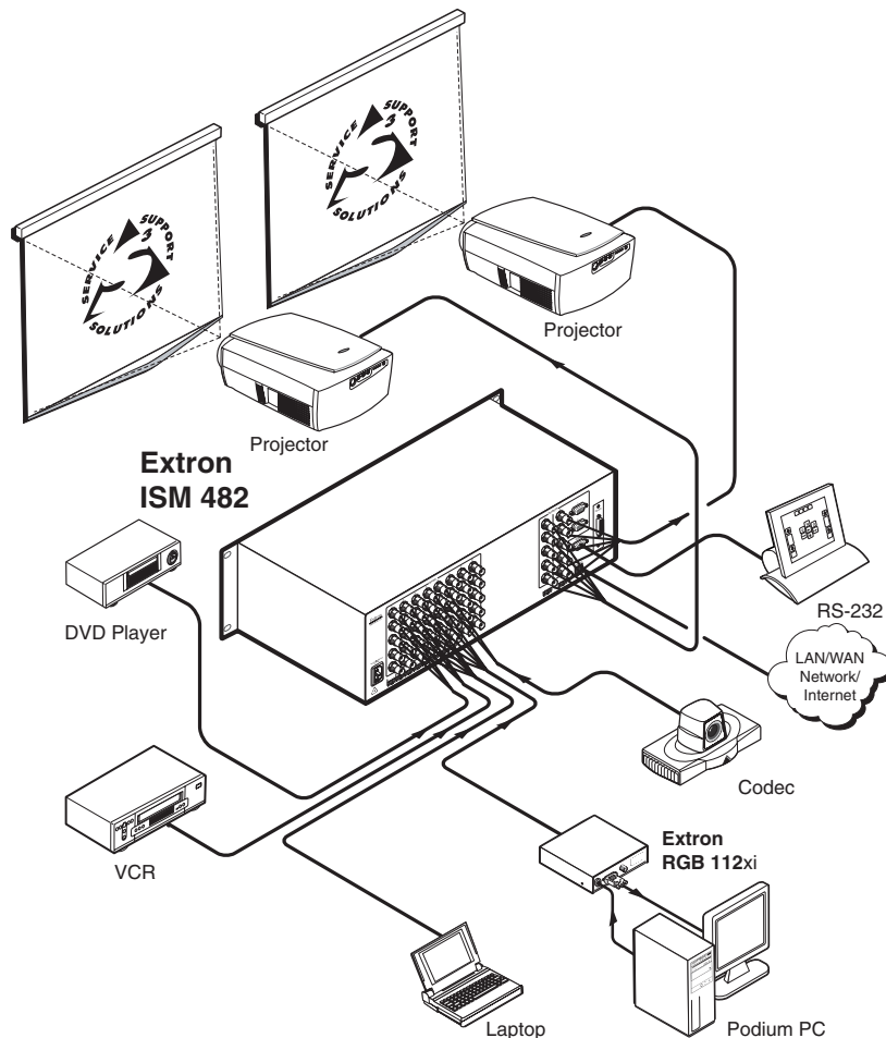
Figure 1-1— Typical ISM 482 Integration Scaling Matrix Switcher application
