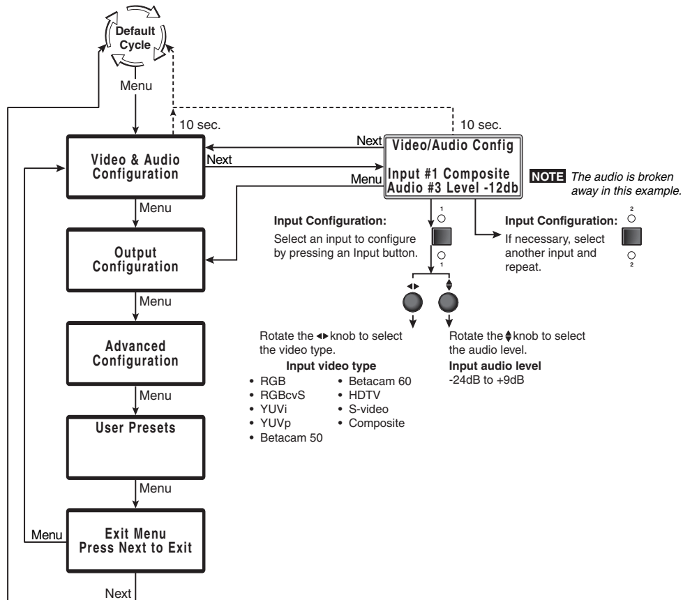
Figure 3-8 — Input Configuration menu flowchart
