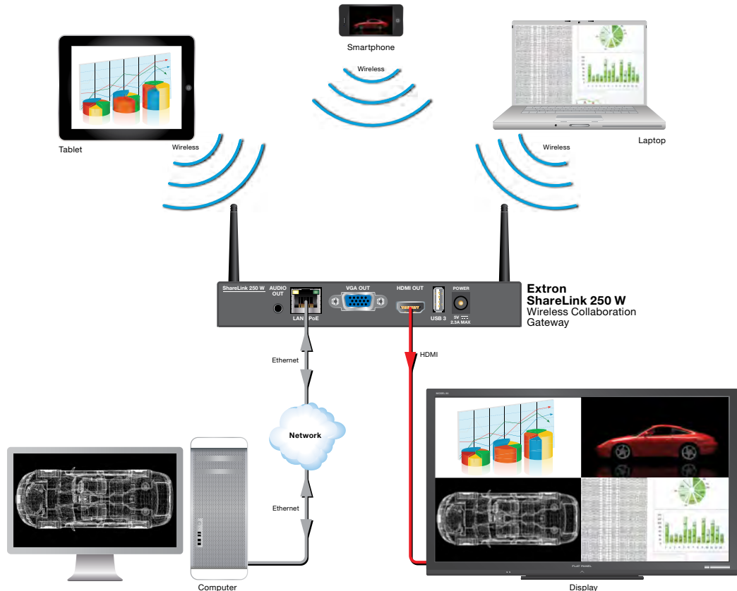
Figure 1. ShareLink 250 W Application Diagram
