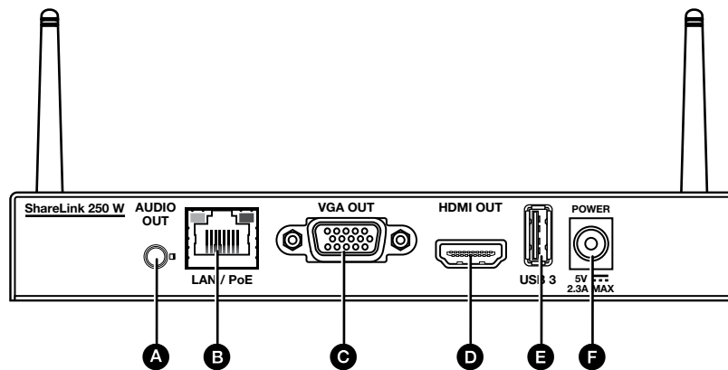
Figure 2. Rear Panel
