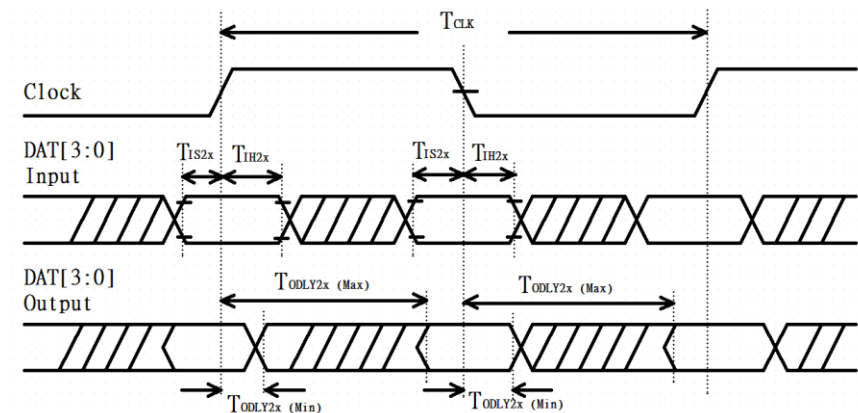
Figure 7: SDIO DAT[3:0] timing Diagram--- SDR50 modes (50 MHz) (1.8V)
