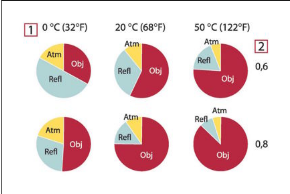
Figure 34.3 Relative magnitudes of radiation sources under varying measurement conditions (SW camera). 1: Object temperature; 2: Emittance; Obj: Object radiation; Refl: Reflected radiation; Atm: atmosphere radiation. Fixed parameters: \tau = 0.88 ; T_{\text{refl}} = 20^{\circ}\text{C} (+68°F); T_{\text{atm}} = 20^{\circ}\text{C} (+68°F).
