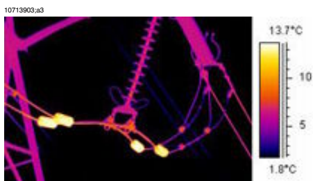
Figure 28.13 An infrared image of hot stabilizing weights
