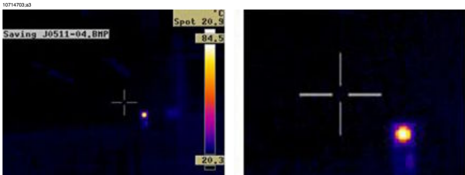
Figure 28.21 Image from the viewfinder of a ThermoCAM 695
