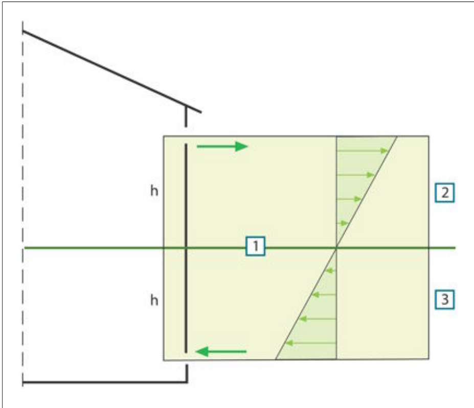
Figure 27.5 Distribution of pressures on a building with two openings and where the external temperature is lower than the internal temperature. 1: Neutral zone; 2: Positive pressure; 3: Negative pressure; h : Distance from the neutral zone in meters.
