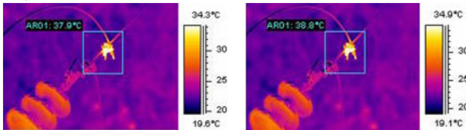
Figure 28.18 LEFT: Incorrect distance setting; RIGHT: Correct distance setting
