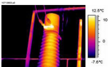
Figure 28.12 An infrared image of a circuit breaker
