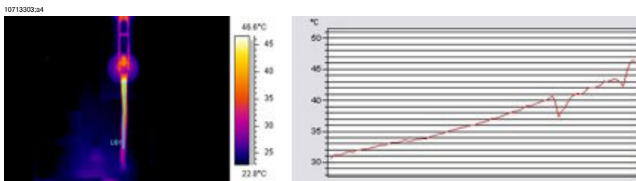
Figure 28.7 A profile (line) in an infrared image and a graph displaying the increasing temperature
