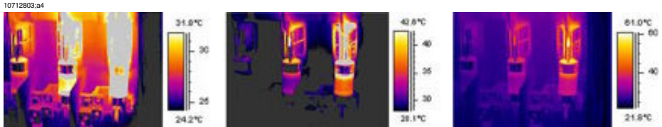
Figure 28.2 Temperature variations in a fusebox
