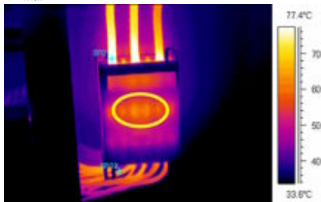
Figure 28.4 A hidden hot spot inside a box
