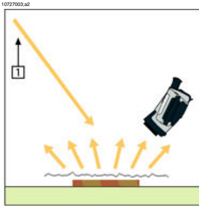
Figure 31.4 Measuring the apparent temperature of the aluminum foil
