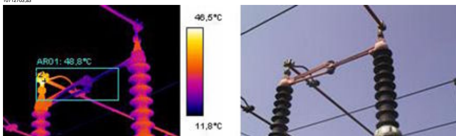
Figure 28.1 An infrared and a visual image of a power line isolator
