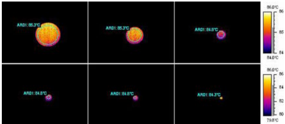
Figure 28.19 Temperature readings from a blackbody at +85°C (+185°F) at increasing distances
