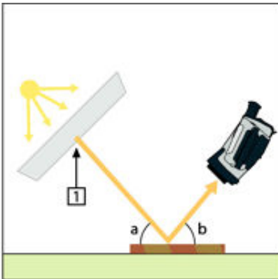
Figure 31.2 1 = Reflection source
