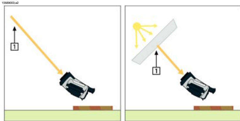
Figure 31.3 1 = Reflection source
