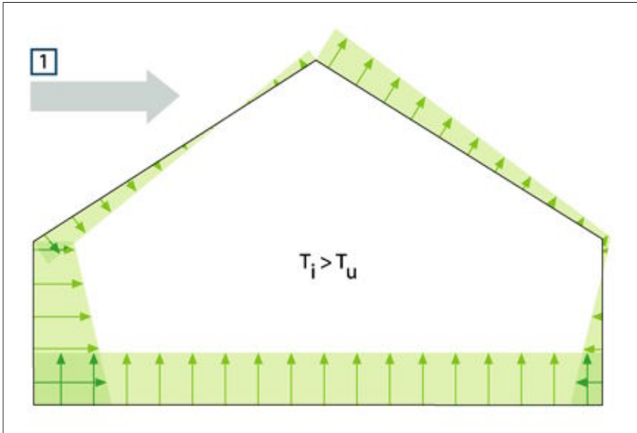
Figure 27.3 Distribution of resultant pressures on a building's enclosing surfaces depending on wind effects, ventilation and internal/external temperature difference. 1: Wind direction; T_u : Thermodynamic air temperature outdoors in K; T_i : Thermodynamic air temperature indoors in K.
