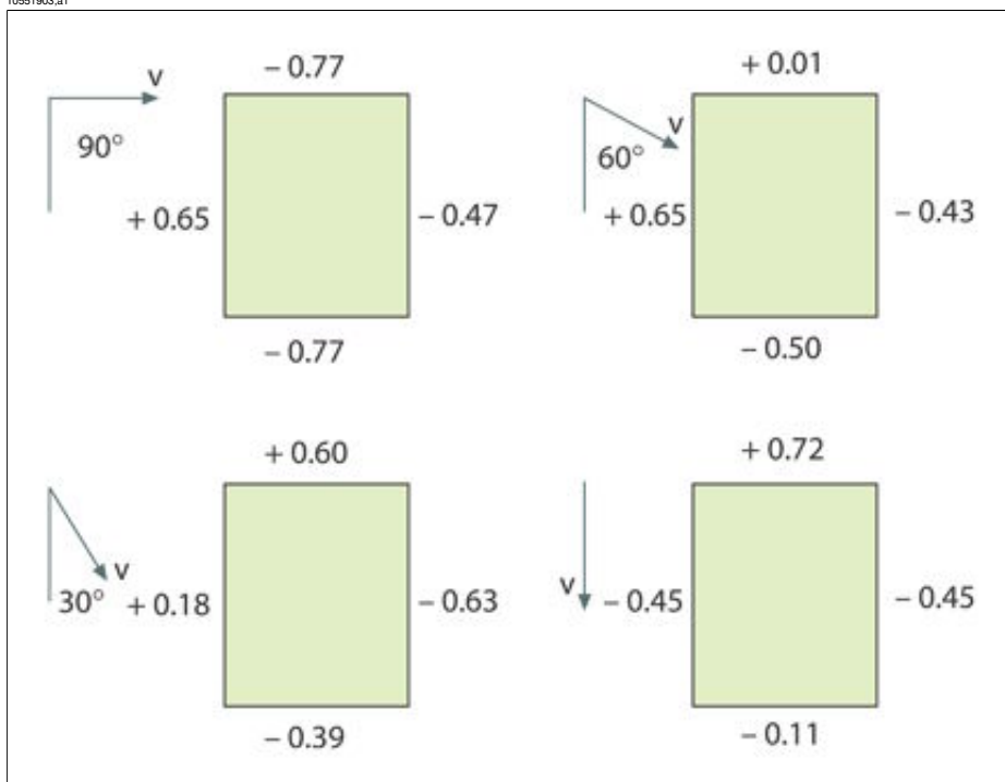
Figure 27.4 Stress concentration factor (C) distributions for various wind directions and wind velocities (v) relative to a building.
