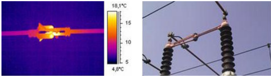
Figure 28.17 Overheating in a circuit breaker
