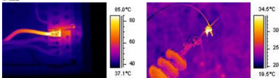
Figure 28.16 LEFT: An infrared image showing bad contact due to a loose bolt; RIGHT: A loose outdoor connection, exposed to the wind cooling effect.
