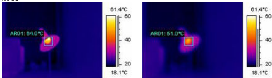
Figure 28.5 LEFT: A hot spot in focus; RIGHT: A hot spot out of focus
