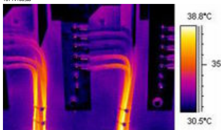
Figure 28.15 An infrared image of bundled cables
