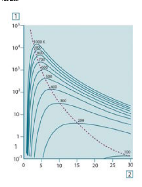
Figure 33.6 Planckian curves plotted on semi-log scales from 100 K to 1000 K. The dotted line represents the locus of maximum radiant emittance at each temperature as described by Wien's displacement law. 1: Spectral radiant emittance ( \text{W}/\text{cm}^2 (\mu\text{m}) ); 2: Wavelength ( \mu\text{m} ).
