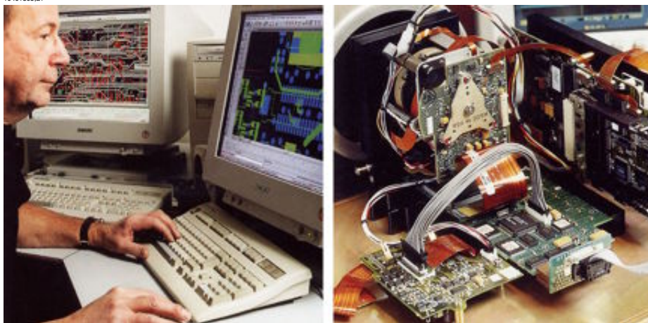
Figure 29.3 LEFT: Development of system electronics; RIGHT: Testing of an FPA detector
