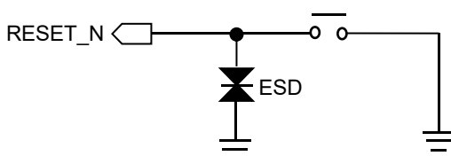
Figure 3.1.3-1 System Reset
