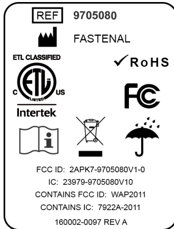
Figure 9. Repeater Label
