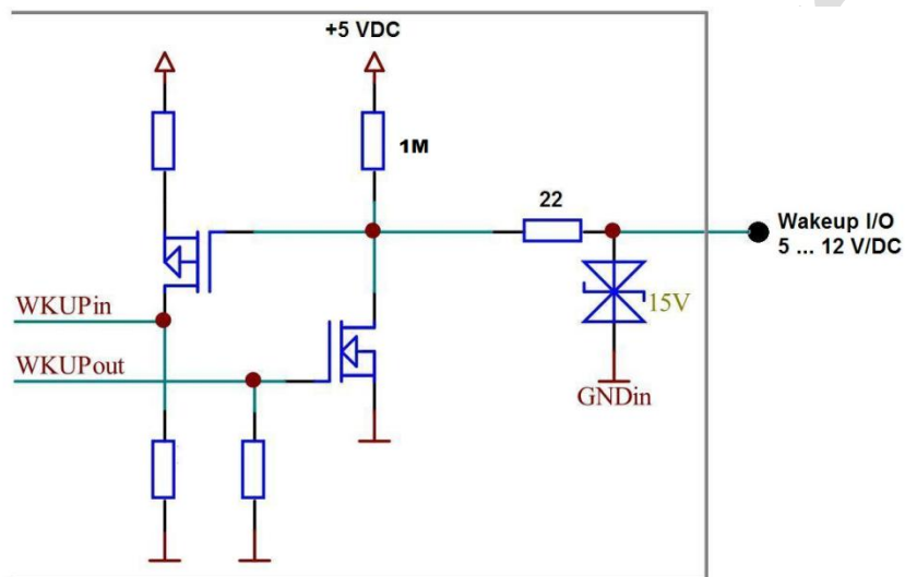
Fig. 15: cVEND internal Wake-up circuit
