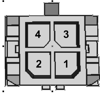
Fig. 12: RS232 V.24 (UART#1) Interface at connector X3
