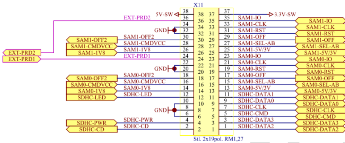
Fig. 17: cVEND plug X11 - PIN assignment.
