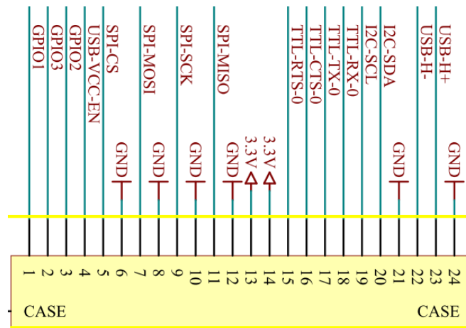
Fig. 21: cVEND plug SAM Extension - X20 Pin assignment
