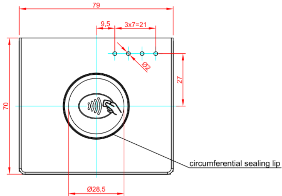
Fig. 6: cVEND plug front with LED position
