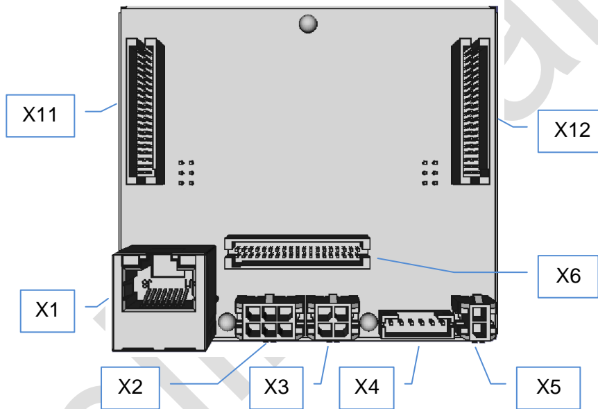
Fig. 1: cVEND plug front view - not installed
