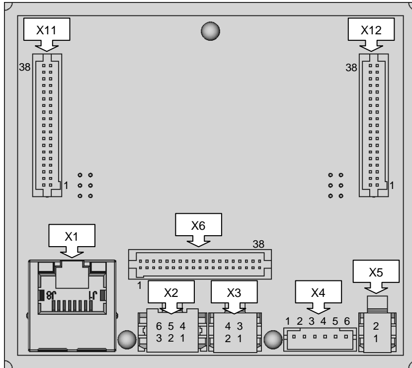
Fig. 8: cVEND plug - connector location
