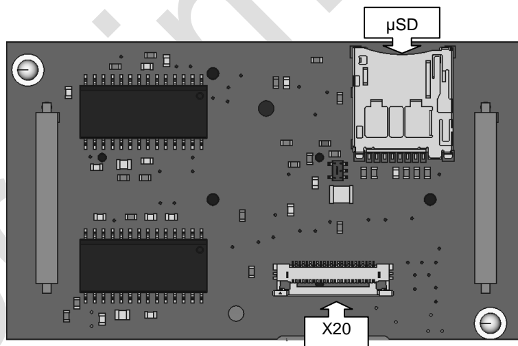
Fig. 20: cVEND plug SAM Extension - bottom view
