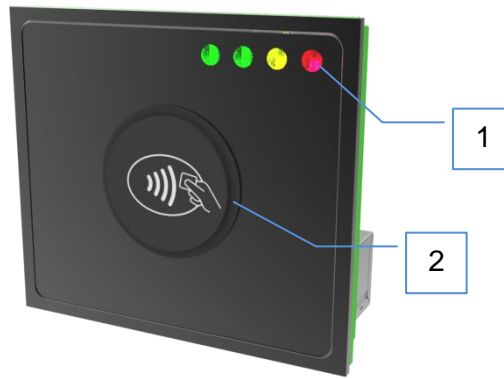
Fig. 1: cVEND plug front view - not installed
