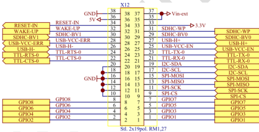
Fig. 18: cVEND plug X12 - PIN assignment.
