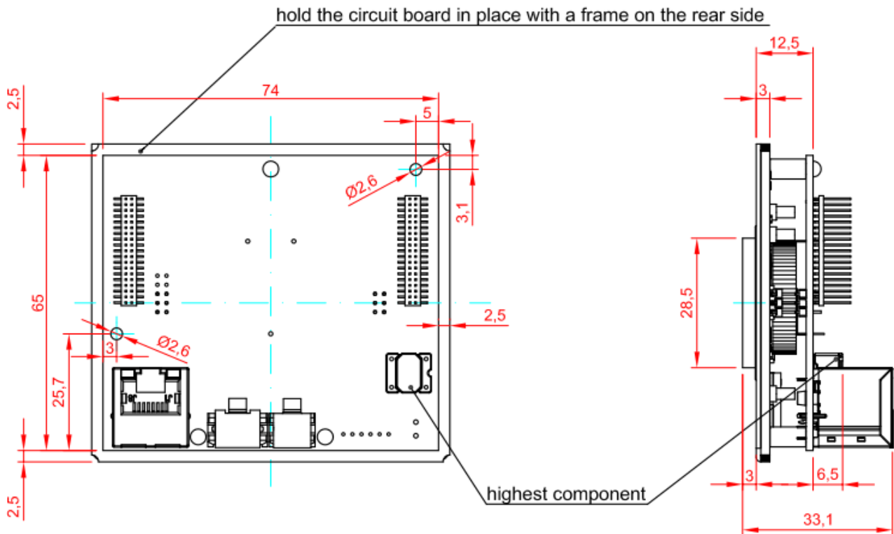
Fig. 7: cVEND plug rear and side view (without cVEND SAM Extension Board)
