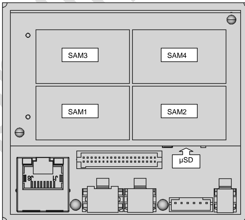
Fig. 9: cVEND plug with optional SAM Extension Board
