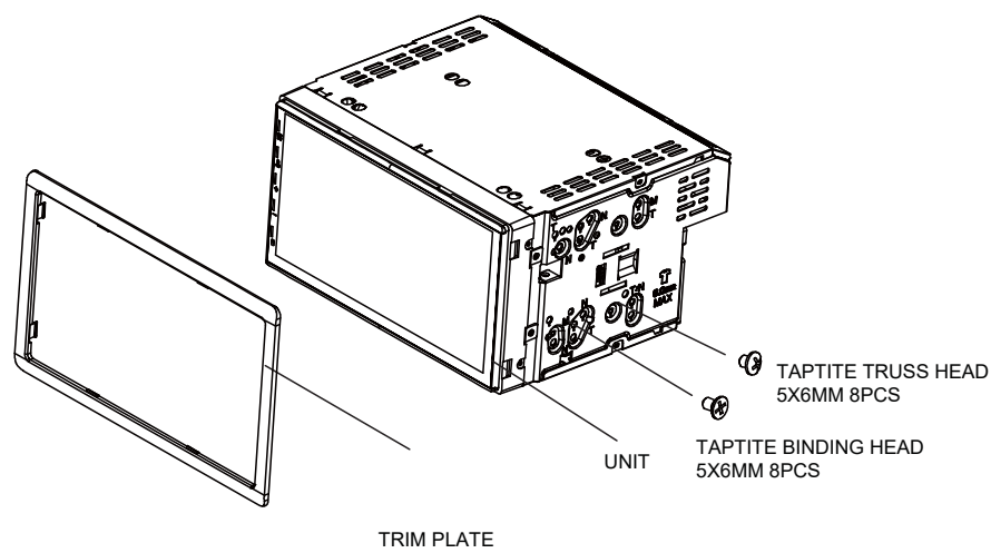
TYPICAL FRONT-LOAD MOUNTING METHOD
