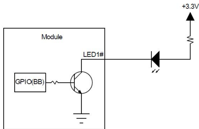
Figure 3-13 LED Driving Circuit
