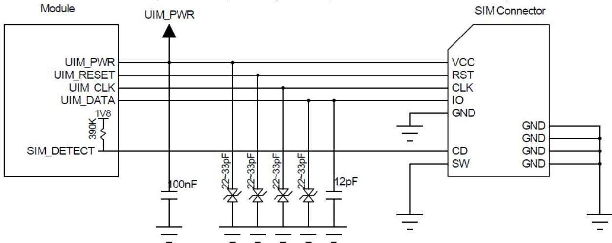
Figure 3-11 Reference Circuit for N.C. SIM Card Slot
