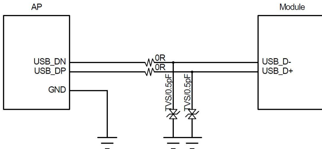
Figure 3-10 Reference Circuit for USB 2.0 Interface
