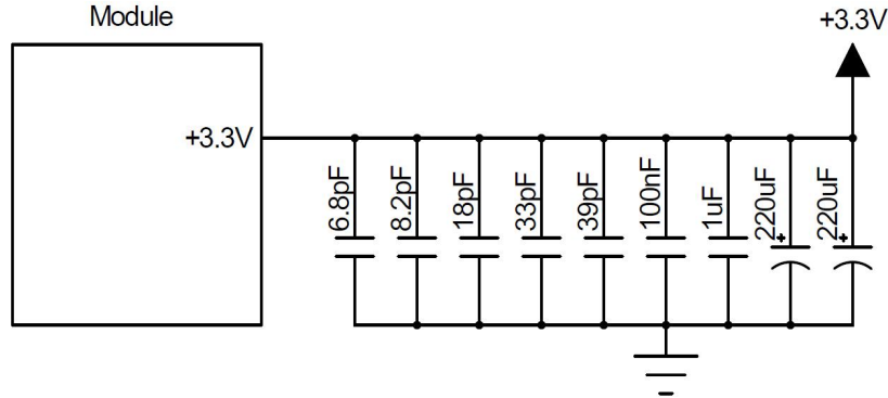
Figure 3-2 Power Supply Design
