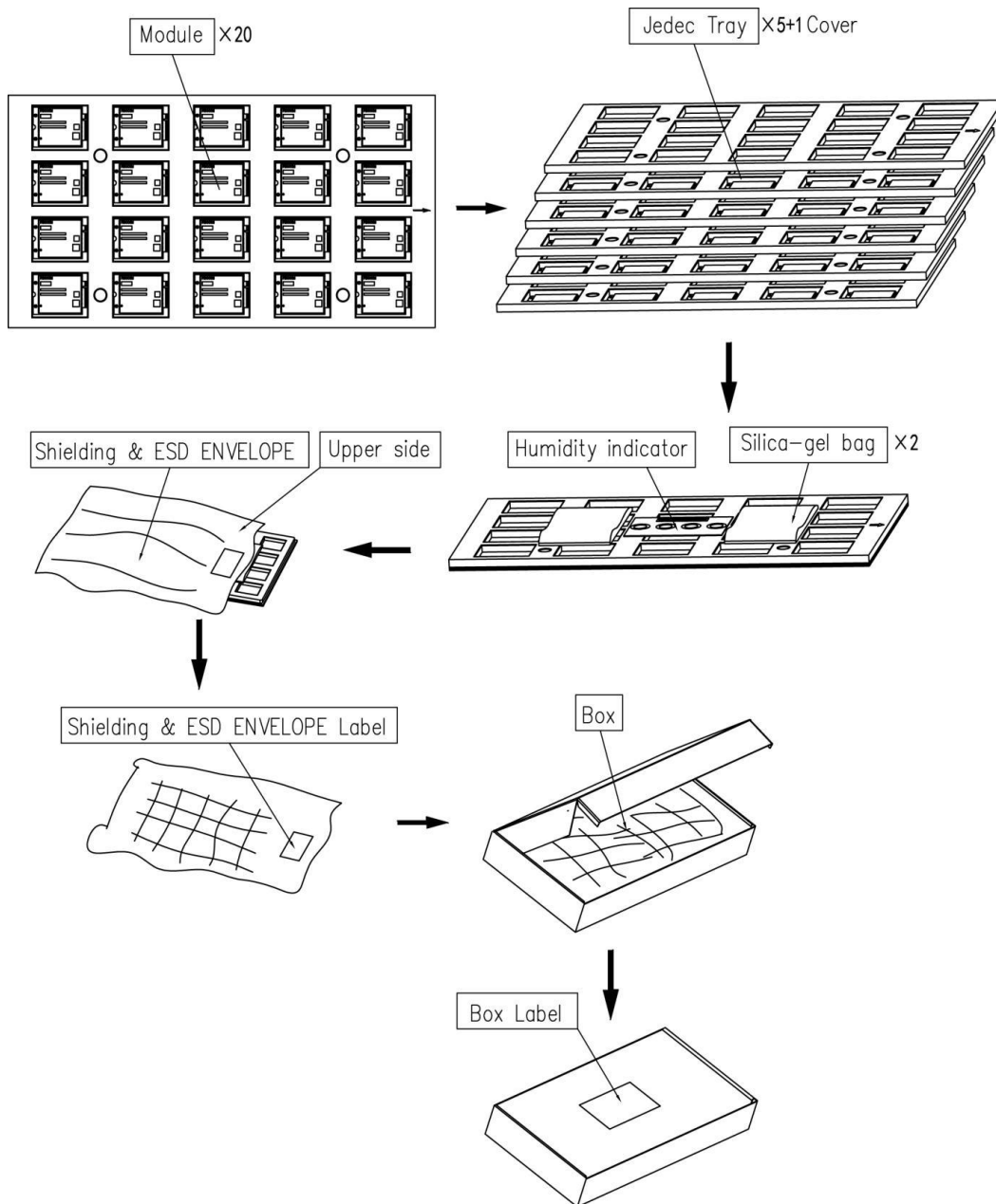
Figure 5-4 Tray Packaging Process
