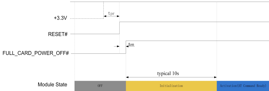
Figure 3-6 Timing Control for Start-up
