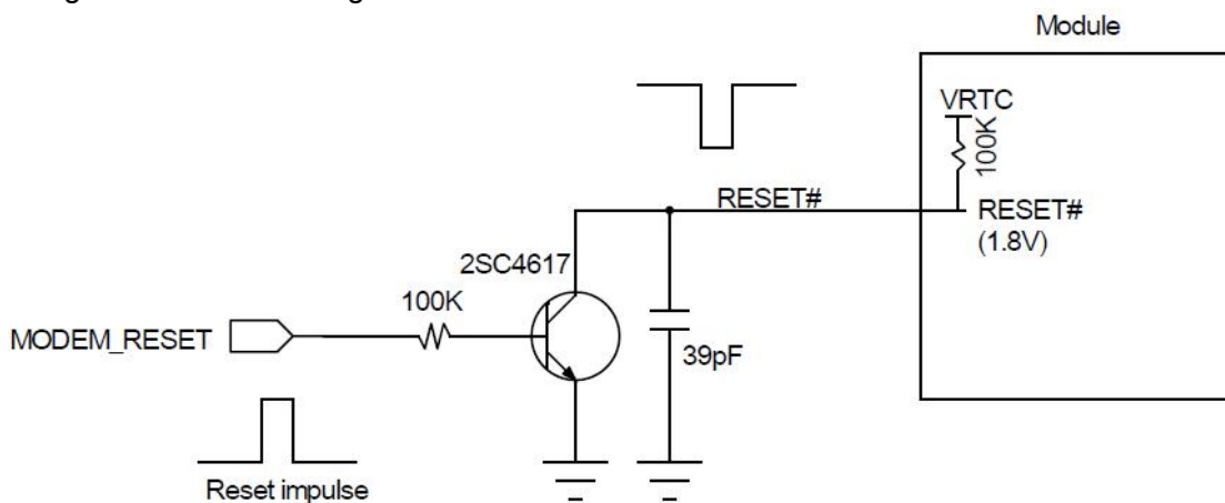
Figure 3-8 Recommended Design for Reset Circuit
