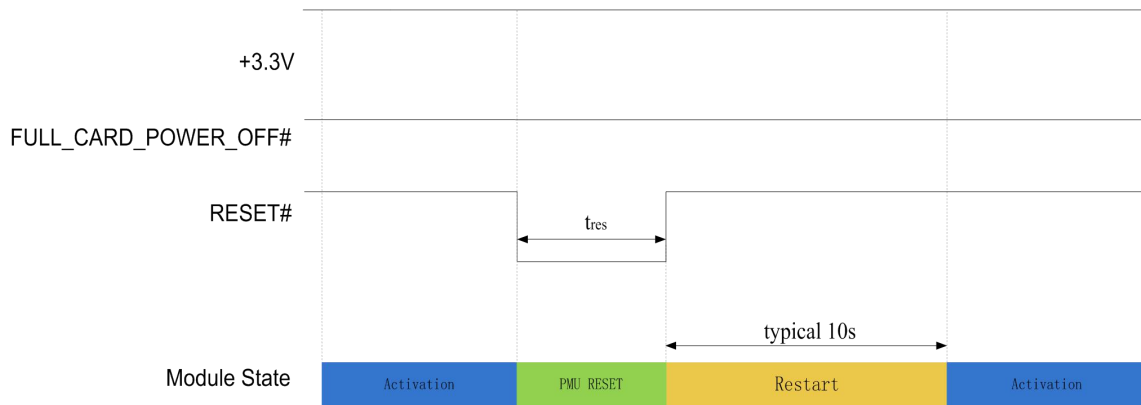
Figure 3-9 Reset Timing Control
