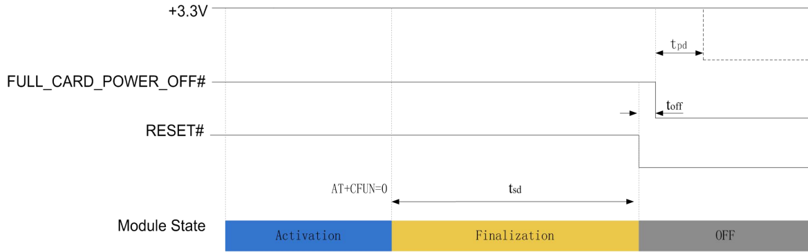
Figure 3-7 Shutdown Timing Control
