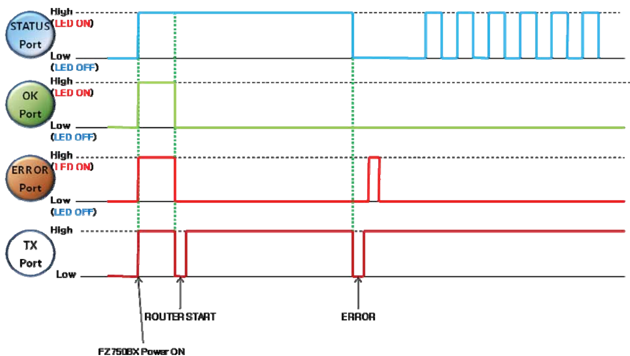
< FZ750BS/FZ750BC is failed to participate in the Zigbee Network/ Operation of Each port >
