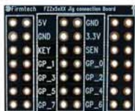
< Figure 7-1-12-⑤ A Extension Interface Connection Board >
