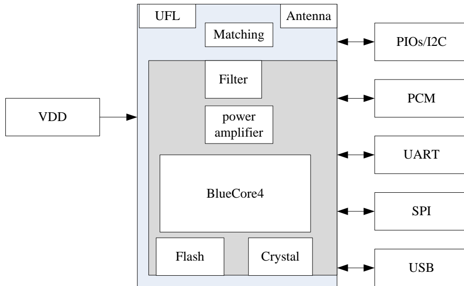
Figure 1: Block Diagram
