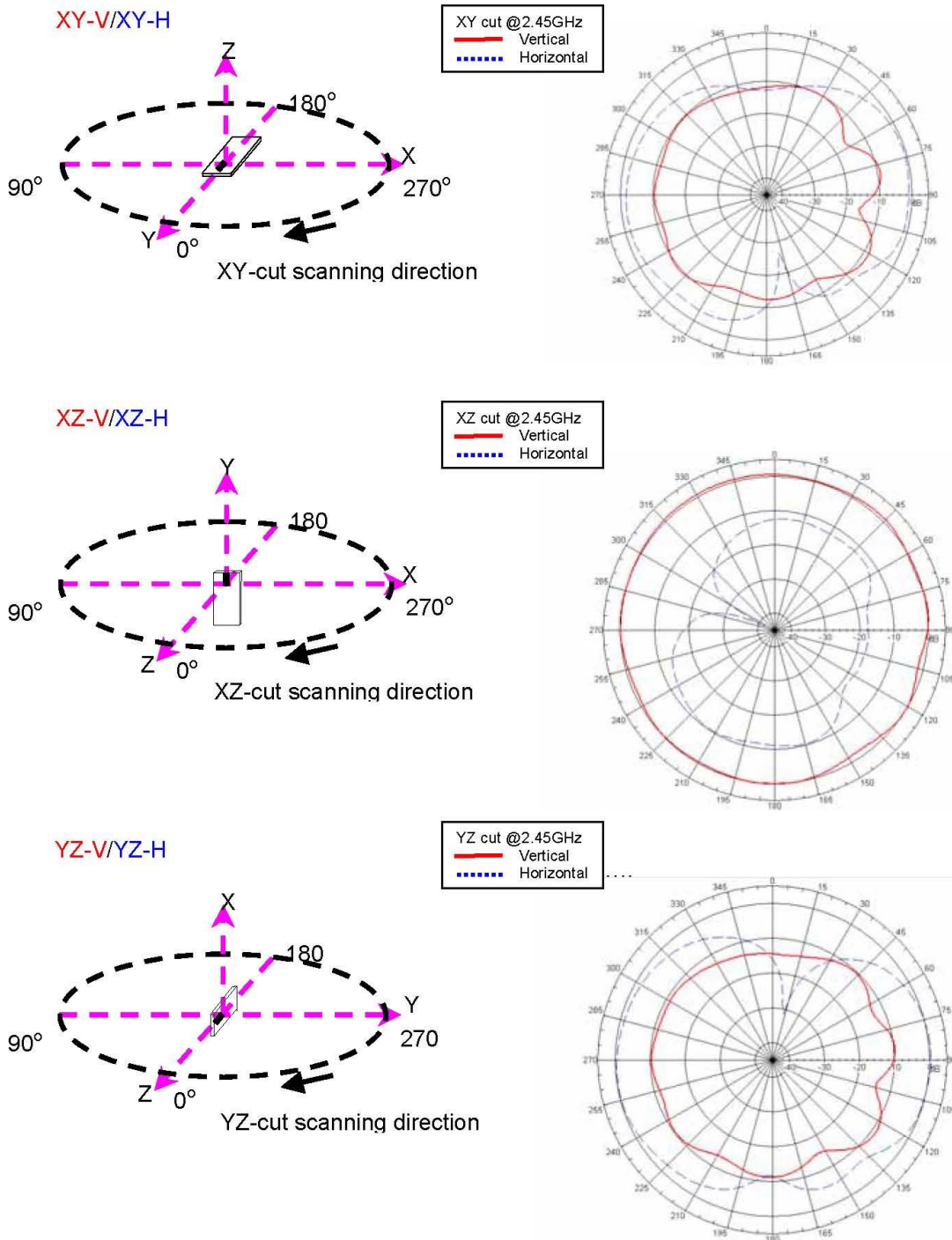
Figure 24: Radiation Patterns of Antenna
