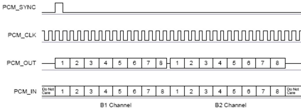
Figure 8: GCI Interface
