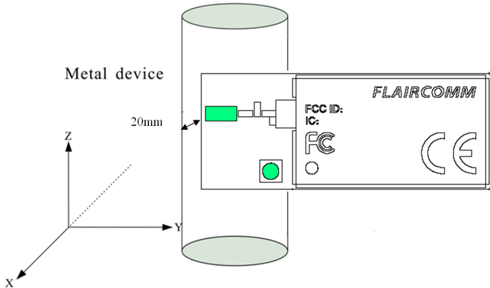
Figure 20: Leave 20mm Clearance Space from the Module Built-in chip Antenna
