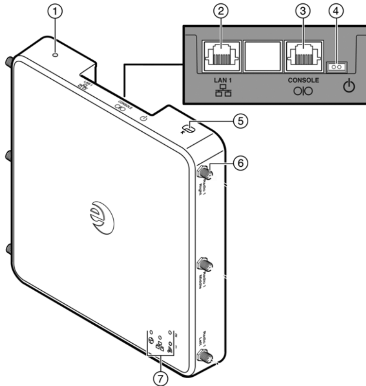
Figure 1-2 Enterasys Wireless AP3710e Front View
