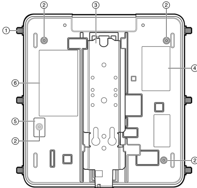
Figure 1-3 WS-AP3710 e Back View
