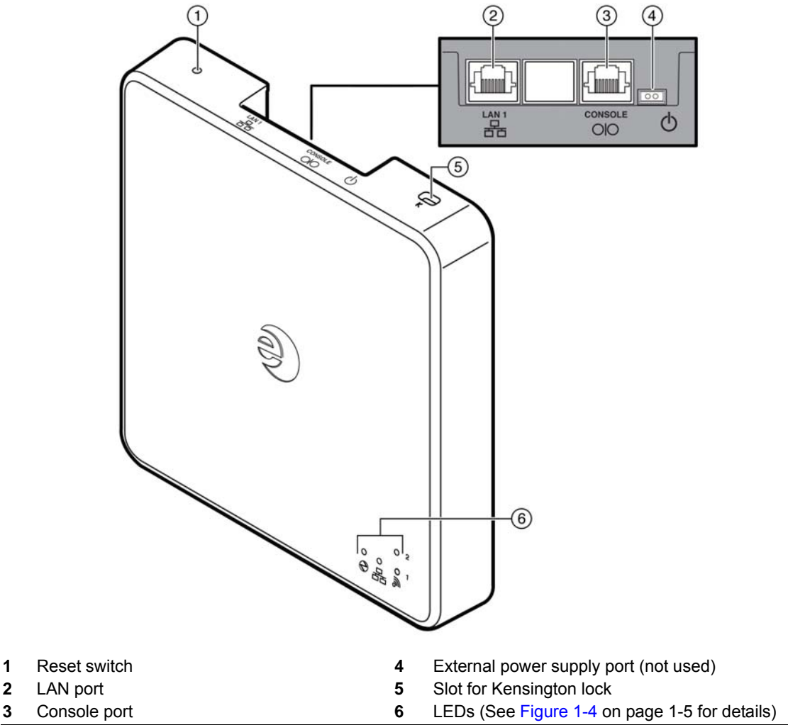
Figure 1-1 Enterasys Wireless AP3710i Front View
