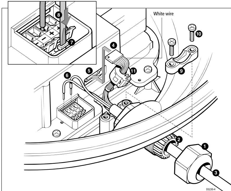
1 Securing nut 2 Gland 3 Inter-unit cable 4 Eight-way plug 5 Eight-way socket 6 Power cores (2 or 4) 7 Terminal clamp 8 Screwdriver 9 Cable clamp 10 Cable clamp screws 11 Ferrite clamp
