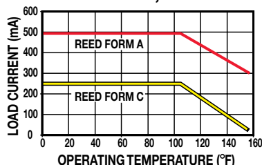
TEMP. vs CURRENT, DC REED
