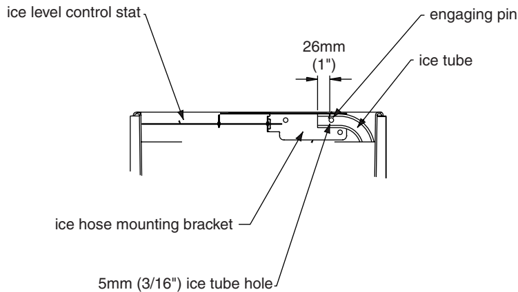
Fig. 6 – Ice transport tube and ice level control stat mounting for freestanding dispensers and countertop units with Satellite-fill icemaker
