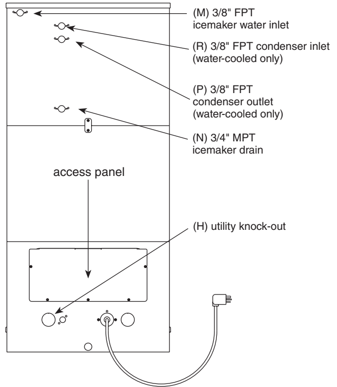
Fig. 5 – Rear connections, countertop models with Satellite-fill icemakers
