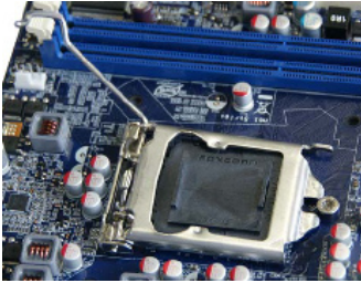
1. Release the CPU socket lever.
