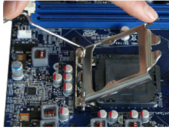
2. Lift the metal cover on the CPU socket.
