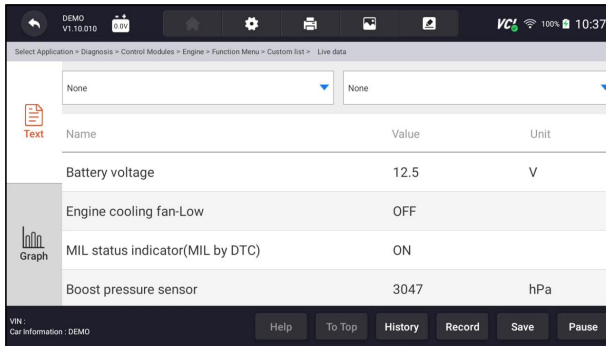
Figure 8-24 Sample Live Data Screen
