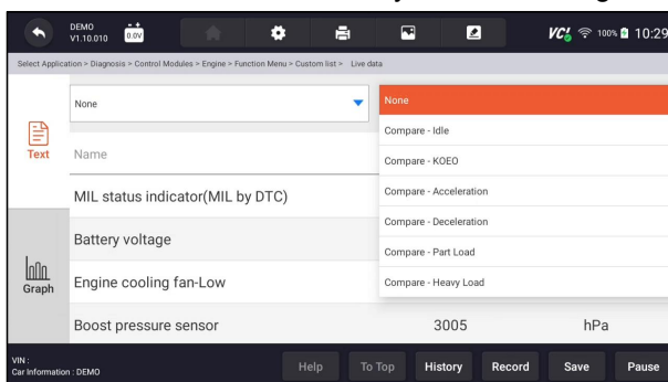
Figure 8-19 Sample Live Data Screen
