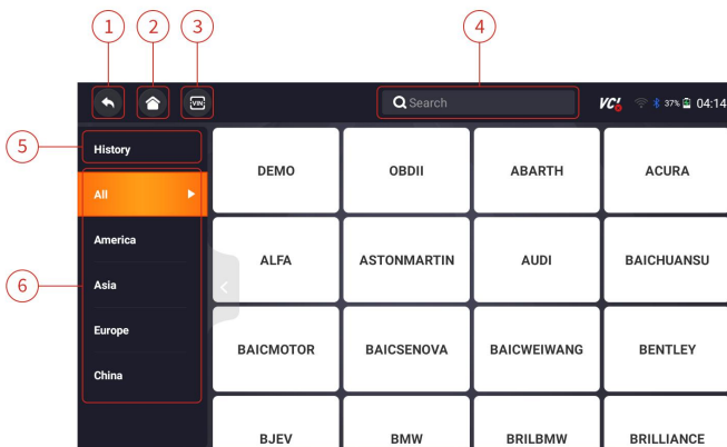
Figure 3-4 Sample Diagnostic Menu Screen
