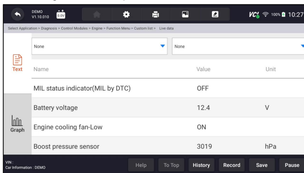
Figure 8-17 Sample Live Data Screen
