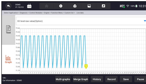
Figure 8-20 Sample PID Graph Screen
