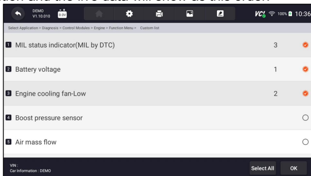
Figure 8-23 Sample Custom List Selection Screen
